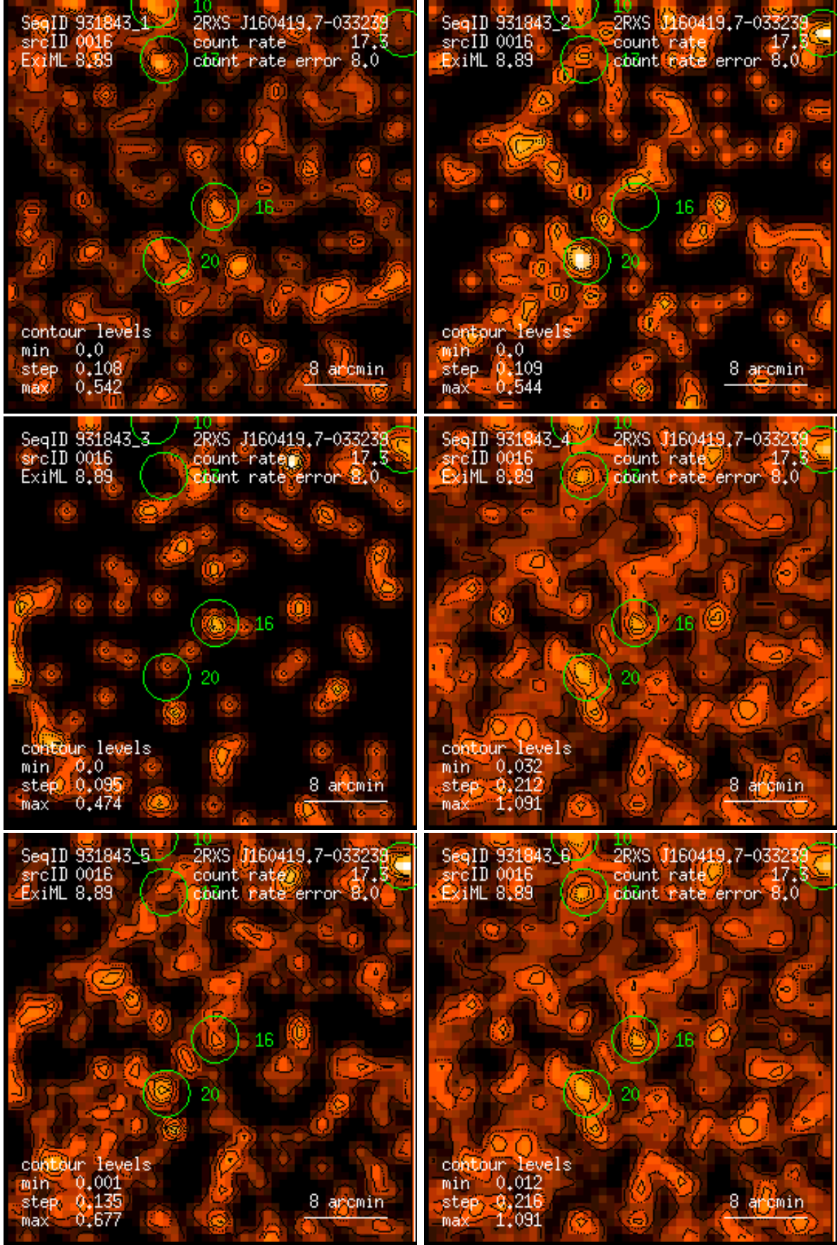
Figure 16: RASS 931843: detection 0016: band rate images, Gaussian filter: (1) PSPC channels 11 – 41, (2) 52 – 90, (3) 91 – 201, (4) 11 – 235, (5) 52 – 201, (6) 11 – 201. Broad band rates in counts/ks. Band rate contour levels in counts/ks/arcmin 2 .
