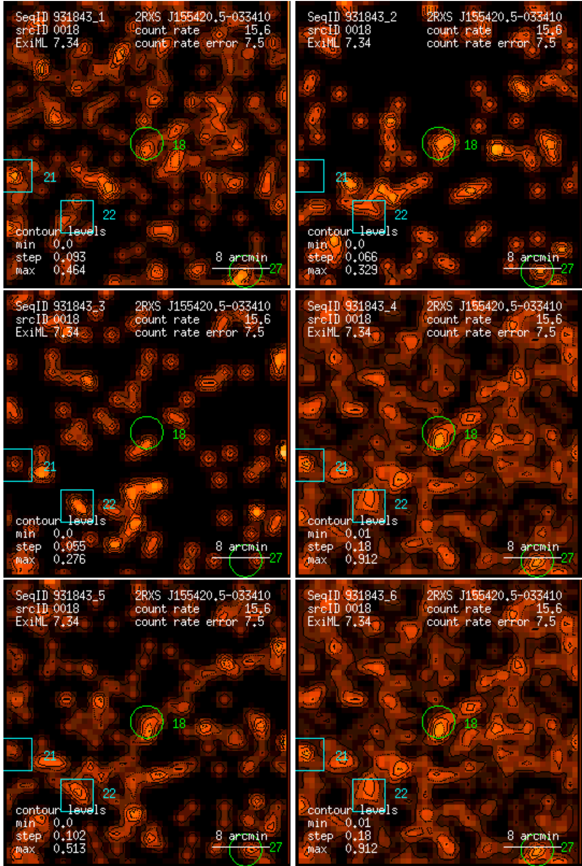
Figure 18: RASS 931843: detection 0018: band rate images, Gaussian filter: (1) PSPC channels 11 – 41, (2) 52 – 90, (3) 91 – 201, (4) 11 – 235, (5) 52 – 201, (6) 11 – 201. Broad band rates in counts/ks. Band rate contour levels in counts/ks/arcmin 2 .
