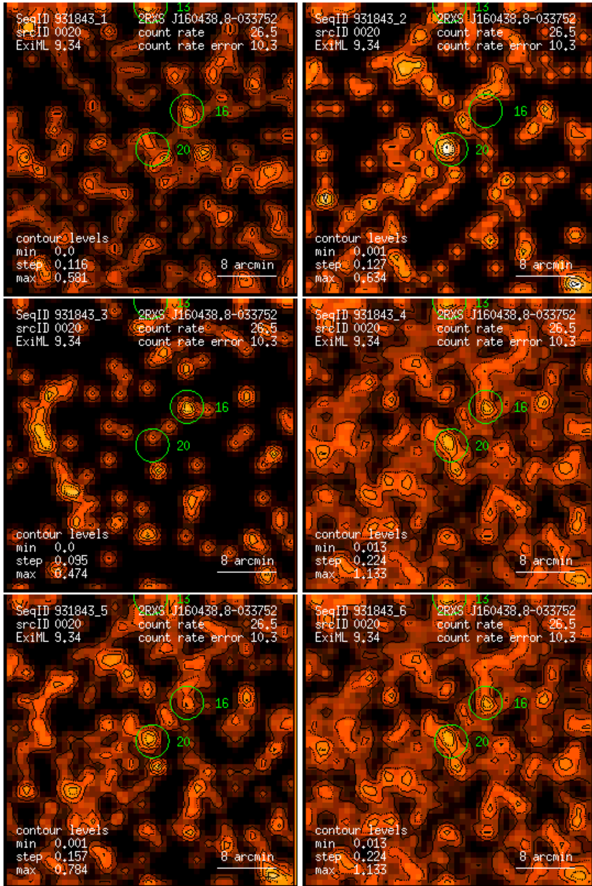
Figure 20: RASS 931843: detection 0020: band rate images, Gaussian filter: (1) PSPC channels 11 – 41, (2) 52 – 90, (3) 91 – 201, (4) 11 – 235, (5) 52 – 201, (6) 11 – 201. Broad band rates in counts/ks. Band rate contour levels in counts/ks/arcmin 2 .
