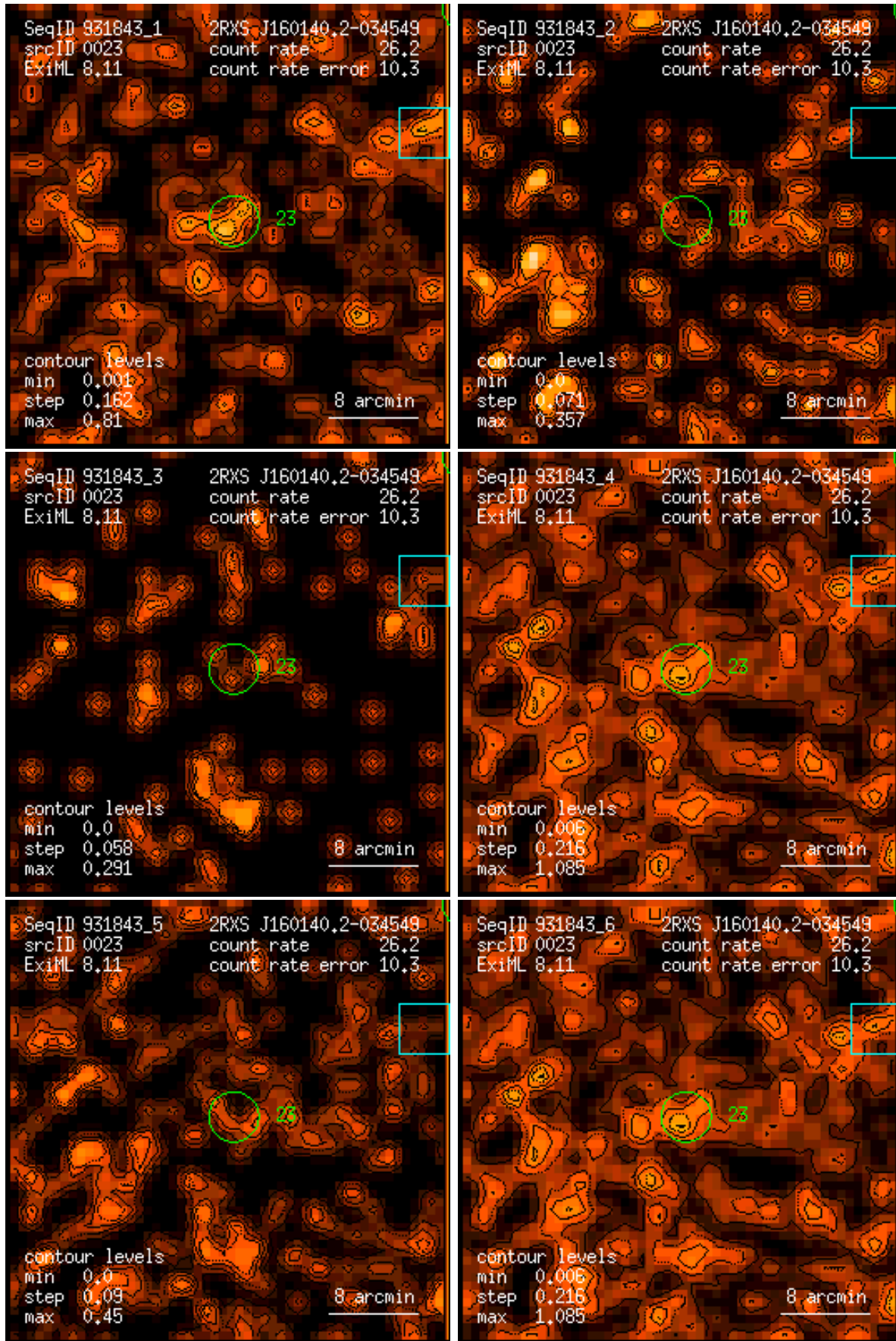
Figure 23: RASS 931843: detection 0023: band rate images, Gaussian filter: (1) PSPC channels 11 – 41, (2) 52 – 90, (3) 91 – 201, (4) 11 – 235, (5) 52 – 201, (6) 11 – 201. Broad band rates in counts/ks. Band rate contour levels in counts/ks/arcmin 2 .
