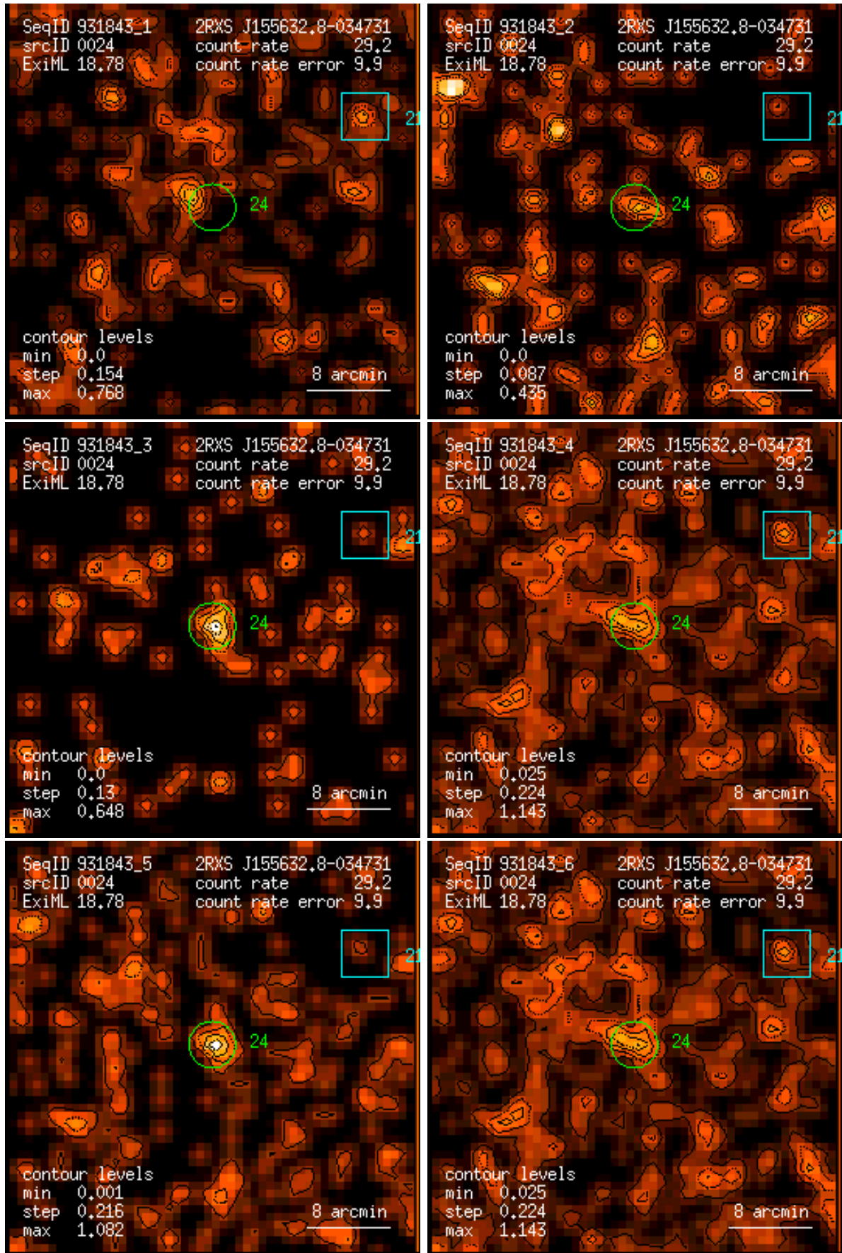
Figure 24: RASS 931843: detection 0024: band rate images, Gaussian filter: (1) PSPC channels 11 – 41, (2) 52 – 90, (3) 91 – 201, (4) 11 – 235, (5) 52 – 201, (6) 11 – 201. Broad band rates in counts/ks. Band rate contour levels in counts/ks/arcmin 2 .
