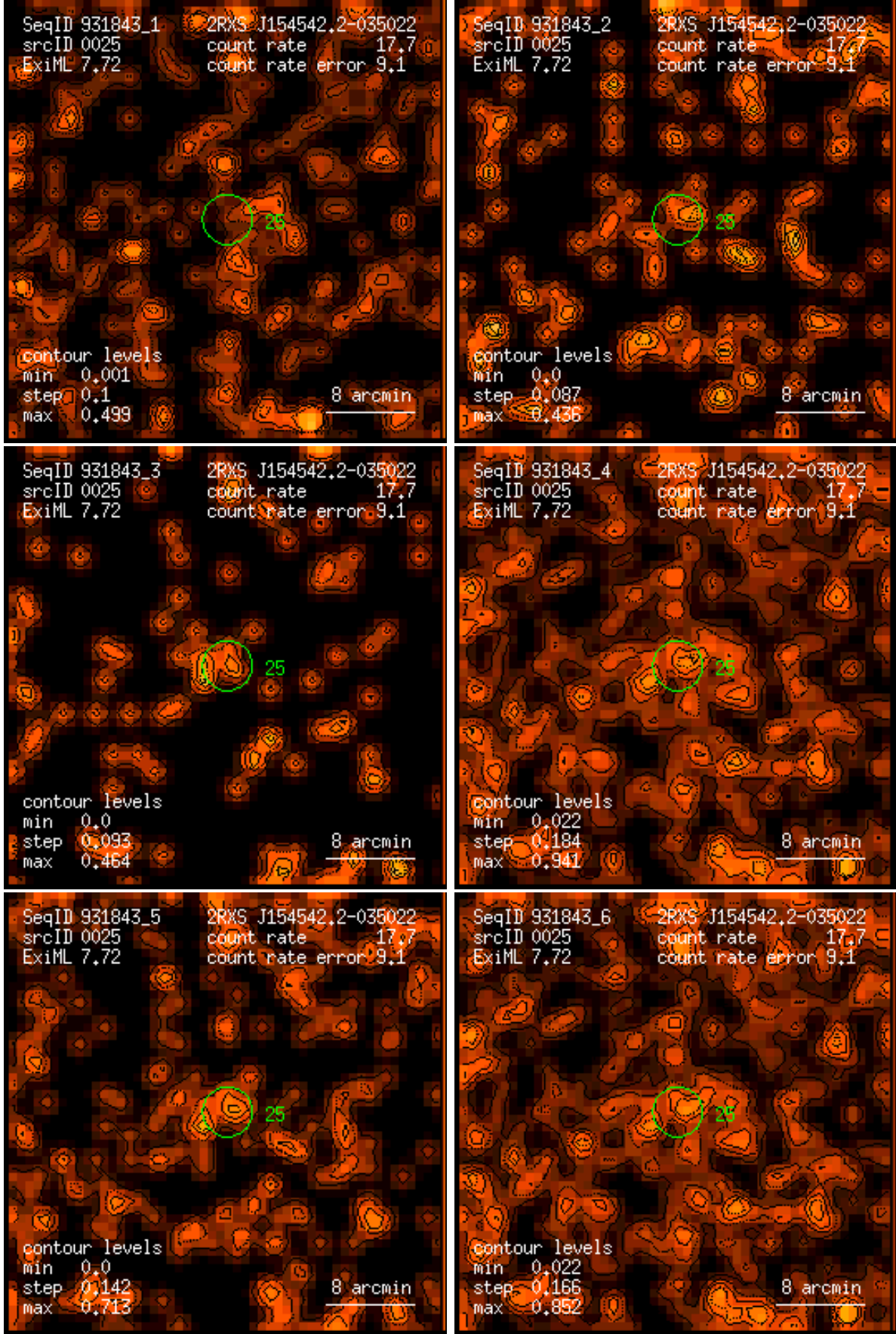
Figure 25: RASS 931843: detection 0025: band rate images, Gaussian filter: (1) PSPC channels 11 – 41, (2) 52 – 90, (3) 91 – 201, (4) 11 – 235, (5) 52 – 201, (6) 11 – 201. Broad band rates in counts/ks. Band rate contour levels in counts/ks/arcmin 2 .
