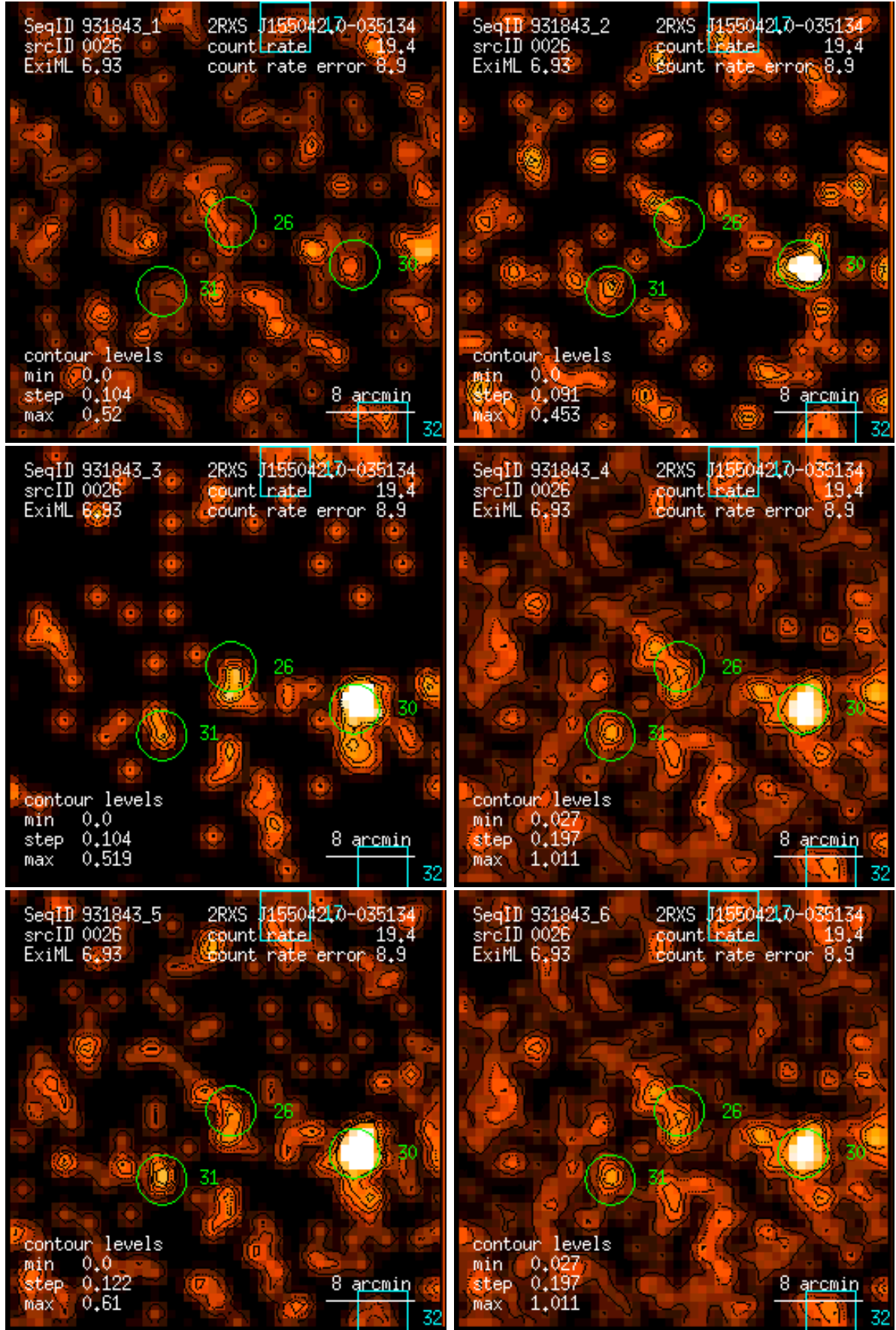
Figure 26: RASS 931843: detection 0026: band rate images, Gaussian filter: (1) PSPC channels 11 – 41, (2) 52 – 90, (3) 91 – 201, (4) 11 – 235, (5) 52 – 201, (6) 11 – 201. Broad band rates in counts/ks. Band rate contour levels in counts/ks/arcmin 2 .
