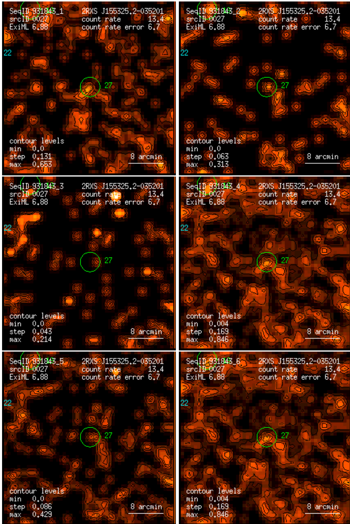
Figure 27: RASS 931843: detection 0027: band rate images, Gaussian filter: (1) PSPC channels 11 – 41, (2) 52 – 90, (3) 91 – 201, (4) 11 – 235, (5) 52 – 201, (6) 11 – 201. Broad band rates in counts/ks. Band rate contour levels in counts/ks/arcmin 2 .
