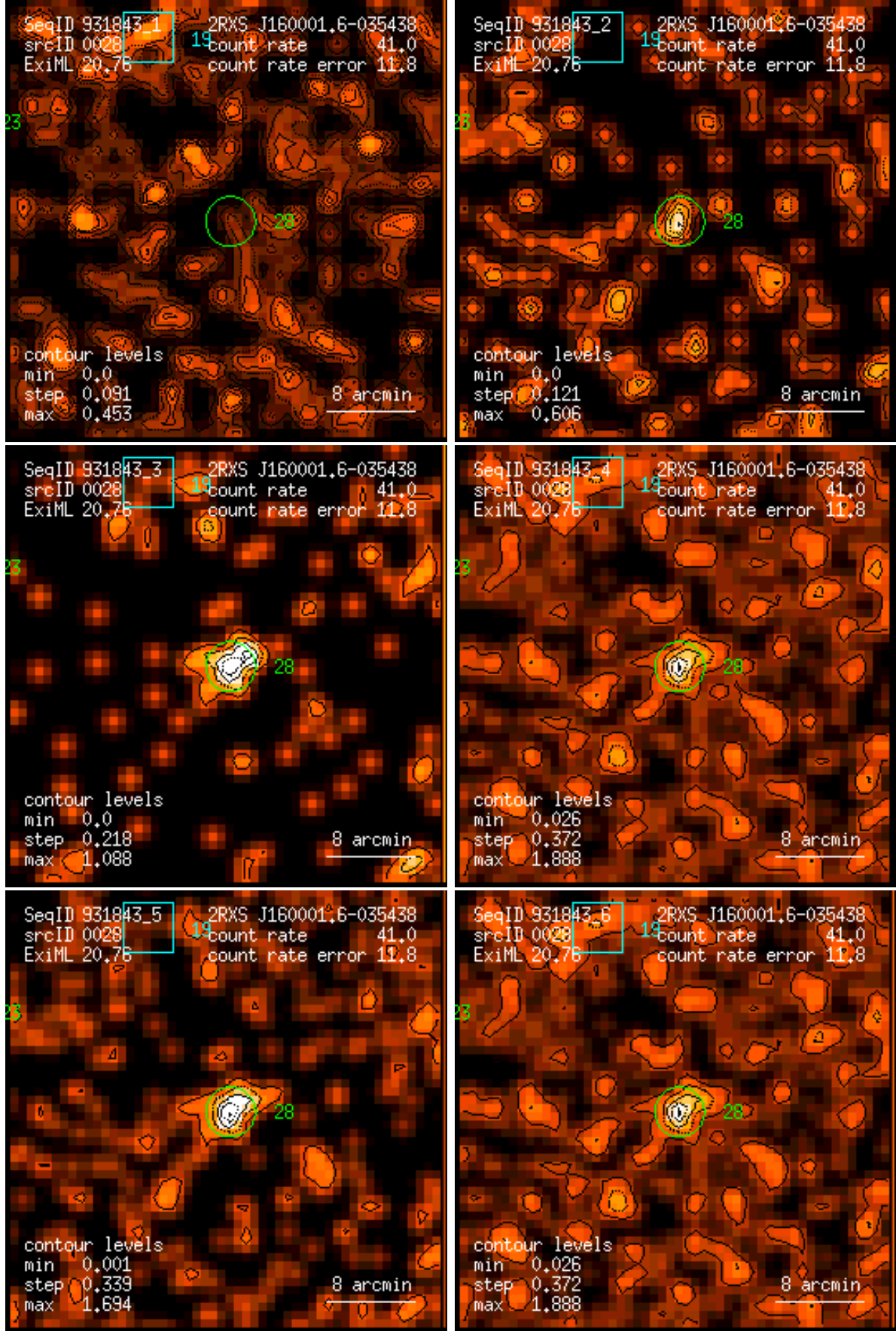
Figure 28: RASS 931843: detection 0028: band rate images, Gaussian filter: (1) PSPC channels 11 – 41, (2) 52 – 90, (3) 91 – 201, (4) 11 – 235, (5) 52 – 201, (6) 11 – 201. Broad band rates in counts/ks. Band rate contour levels in counts/ks/arcmin 2 .
