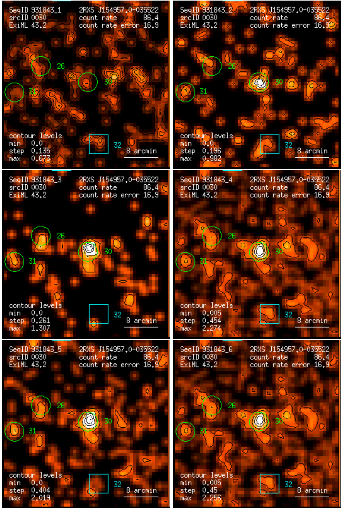
Figure 30: RASS 931843: detection 0030: band rate images, Gaussian filter: (1) PSPC channels 11 – 41, (2) 52 – 90, (3) 91 – 201, (4) 11 – 235, (5) 52 – 201, (6) 11 – 201. Broad band rates in counts/ks. Band rate contour levels in counts/ks/arcmin 2 .
