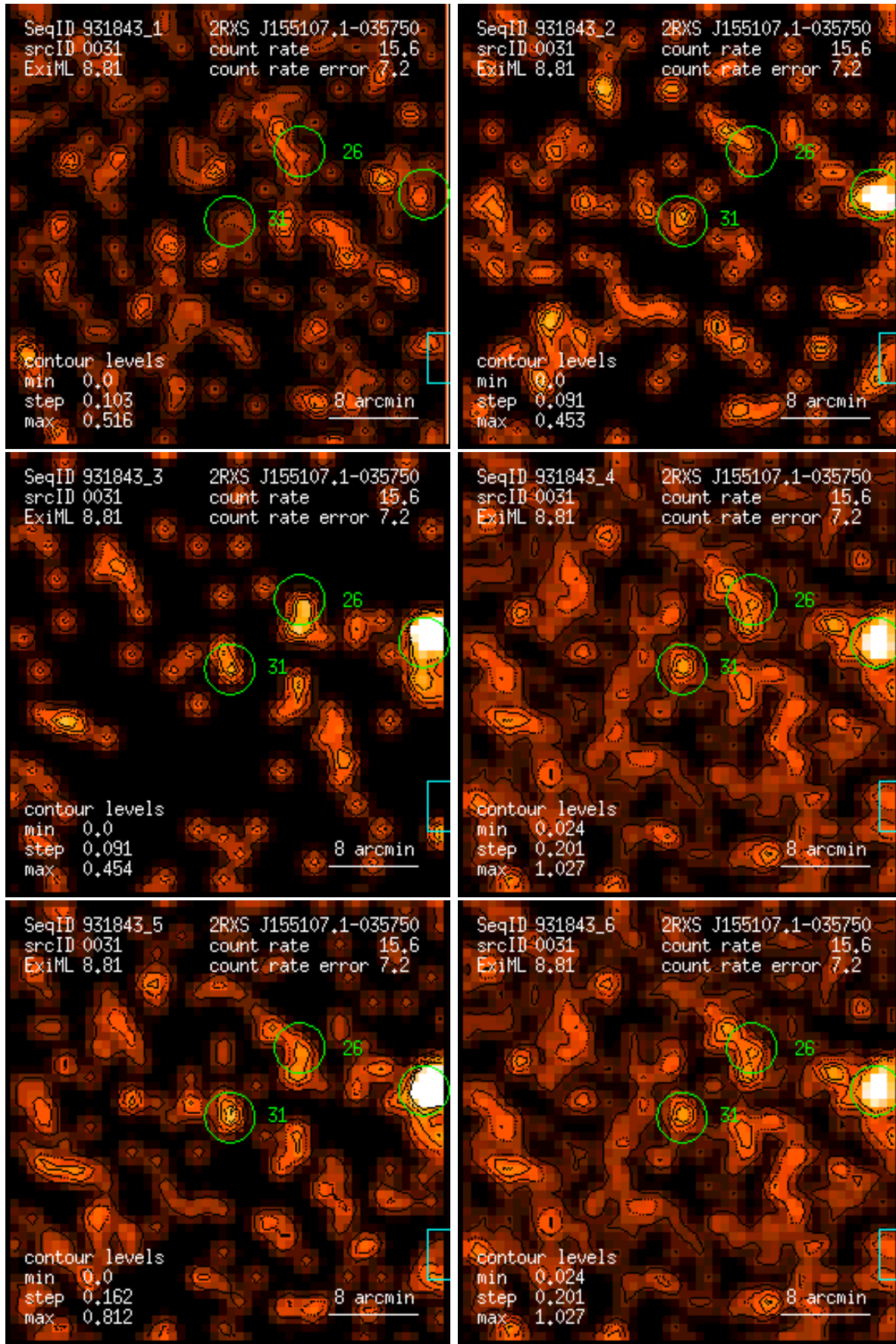
Figure 31: RASS 931843: detection 0031: band rate images, Gaussian filter: (1) PSPC channels 11 – 41, (2) 52 – 90, (3) 91 – 201, (4) 11 – 235, (5) 52 – 201, (6) 11 – 201. Broad band rates in counts/ks. Band rate contour levels in counts/ks/arcmin 2 .
