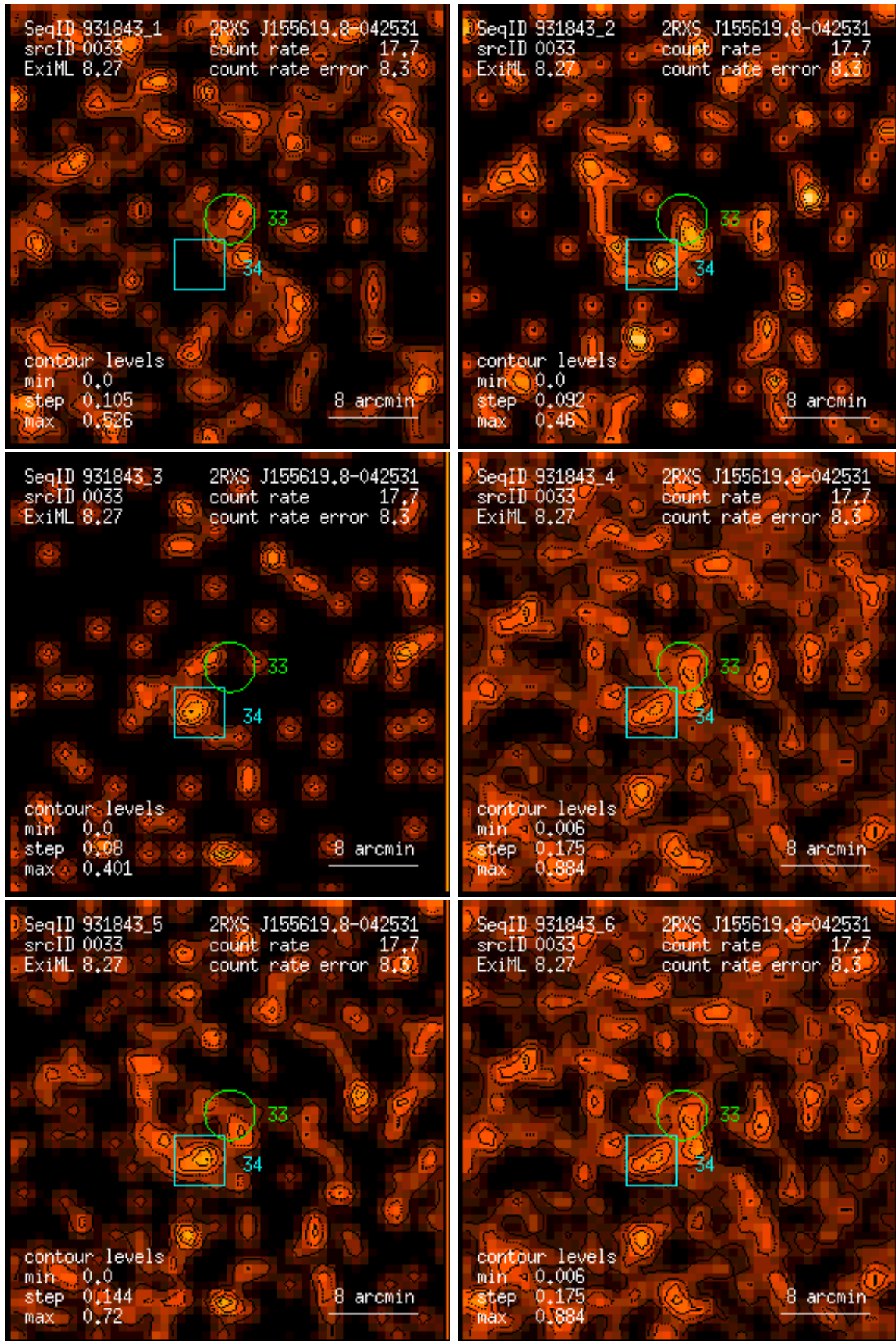
Figure 33: RASS 931843: detection 0033: band rate images, Gaussian filter: (1) PSPC channels 11 – 41, (2) 52 – 90, (3) 91 – 201, (4) 11 – 235, (5) 52 – 201, (6) 11 – 201. Broad band rates in counts/ks. Band rate contour levels in counts/ks/arcmin 2 .
