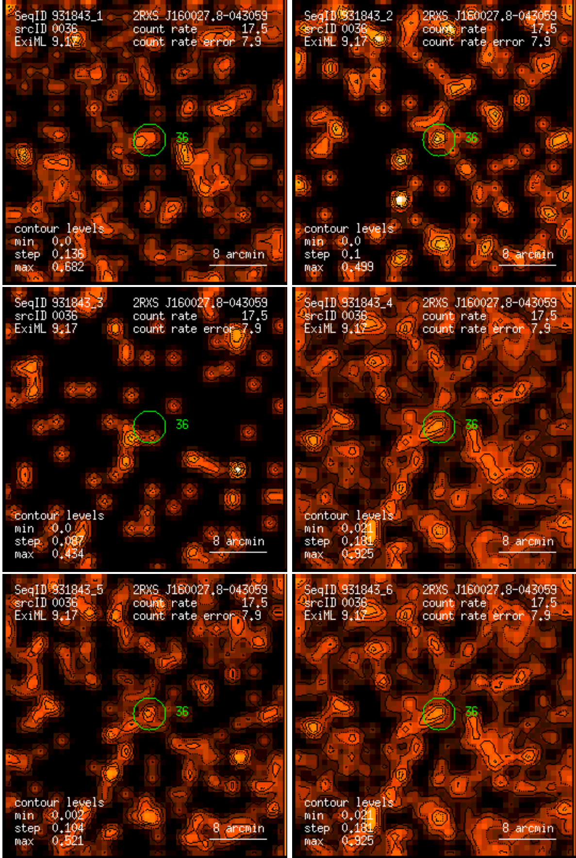
Figure 36: RASS 931843: detection 0036: band rate images, Gaussian filter: (1) PSPC channels 11 – 41, (2) 52 – 90, (3) 91 – 201, (4) 11 – 235, (5) 52 – 201, (6) 11 – 201. Broad band rates in counts/ks. Band rate contour levels in counts/ks/arcmin 2 .
