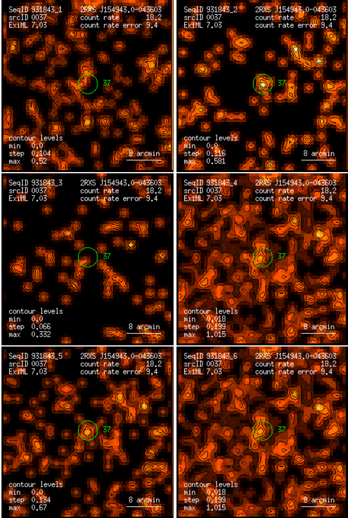
Figure 37: RASS 931843: detection 0037: band rate images, Gaussian filter: (1) PSPC channels 11 – 41, (2) 52 – 90, (3) 91 – 201, (4) 11 – 235, (5) 52 – 201, (6) 11 – 201. Broad band rates in counts/ks. Band rate contour levels in counts/ks/arcmin 2 .
