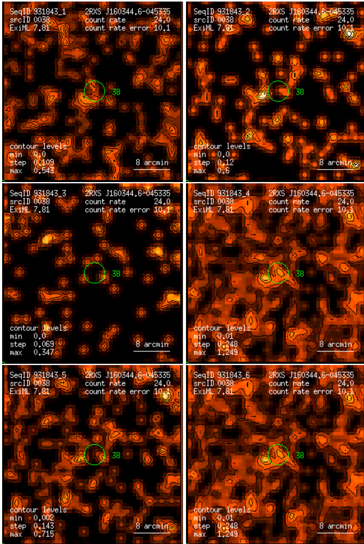
Figure 38: RASS 931843: detection 0038: band rate images, Gaussian filter: (1) PSPC channels 11 – 41, (2) 52 – 90, (3) 91 – 201, (4) 11 – 235, (5) 52 – 201, (6) 11 – 201. Broad band rates in counts/ks. Band rate contour levels in counts/ks/arcmin 2 .
