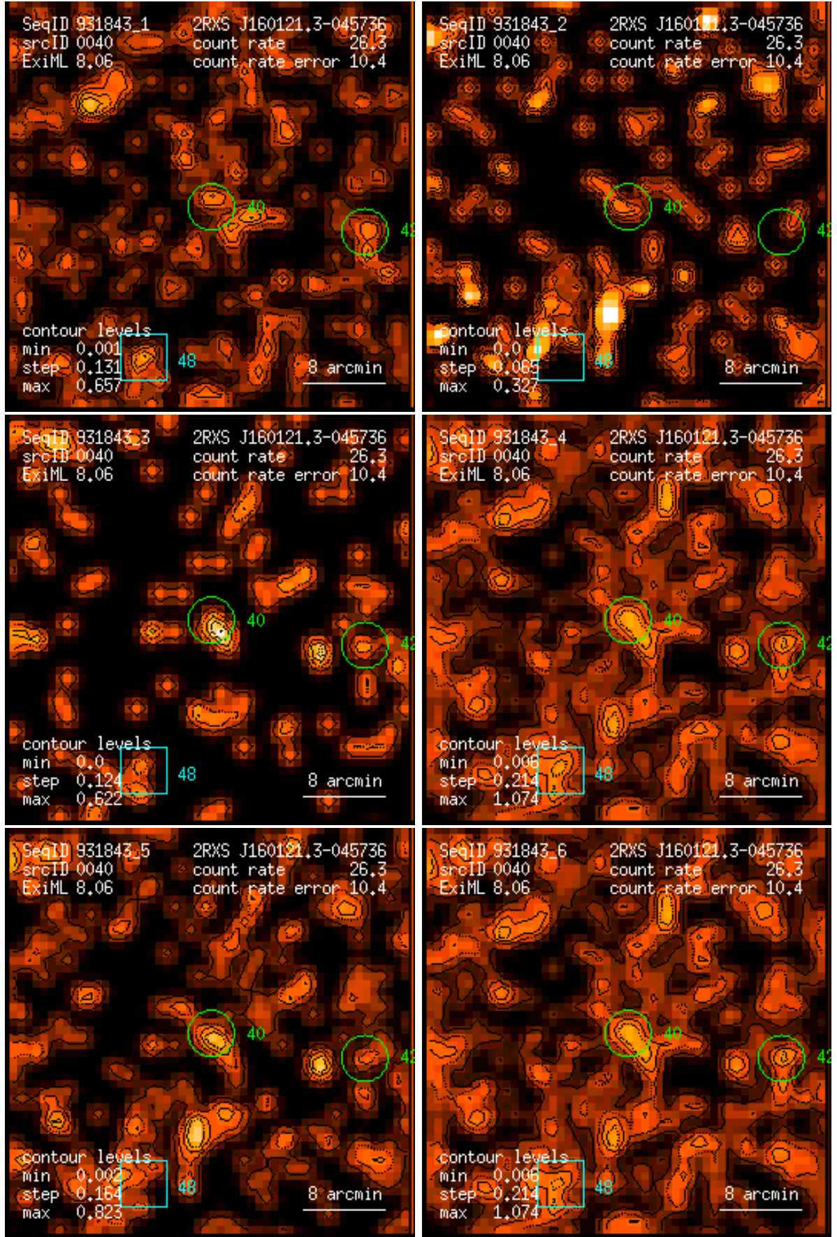
Figure 40: RASS 931843: detection 0040: band rate images, Gaussian filter: (1) PSPC channels 11 – 41, (2) 52 – 90, (3) 91 – 201, (4) 11 – 235, (5) 52 – 201, (6) 11 – 201. Broad band rates in counts/ks. Band rate contour levels in counts/ks/arcmin 2 .
