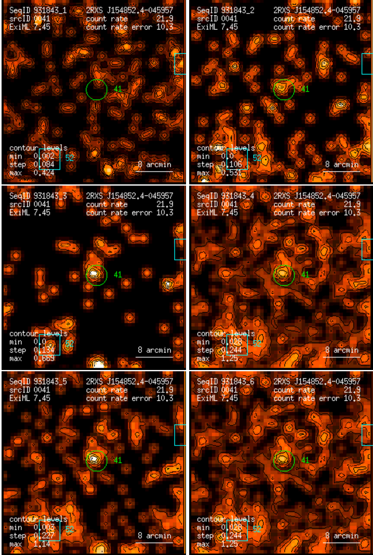
Figure 41: RASS 931843: detection 0041: band rate images, Gaussian filter: (1) PSPC channels 11 – 41, (2) 52 – 90, (3) 91 – 201, (4) 11 – 235, (5) 52 – 201, (6) 11 – 201. Broad band rates in counts/ks. Band rate contour levels in counts/ks/arcmin 2 .
