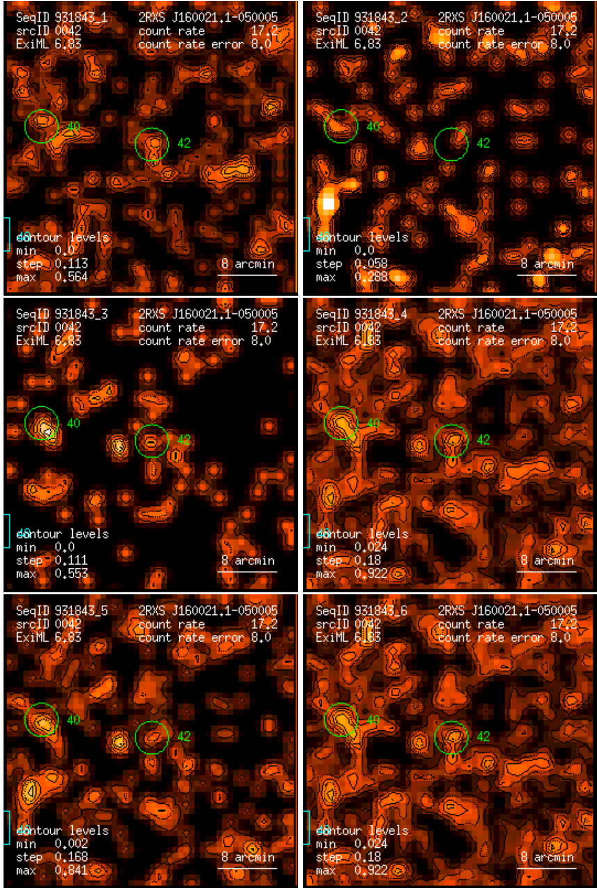
Figure 42: RASS 931843: detection 0042: band rate images, Gaussian filter: (1) PSPC channels 11 – 41, (2) 52 – 90, (3) 91 – 201, (4) 11 – 235, (5) 52 – 201, (6) 11 – 201. Broad band rates in counts/ks. Band rate contour levels in counts/ks/arcmin 2 .
