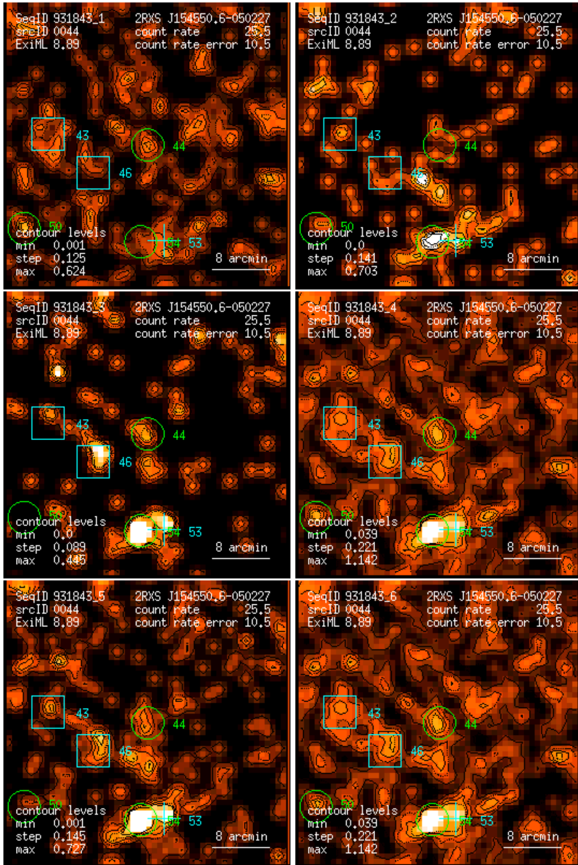
Figure 44: RASS 931843: detection 0044: band rate images, Gaussian filter: (1) PSPC channels 11 – 41, (2) 52 – 90, (3) 91 – 201, (4) 11 – 235, (5) 52 – 201, (6) 11 – 201. Broad band rates in counts/ks. Band rate contour levels in counts/ks/arcmin 2 .
