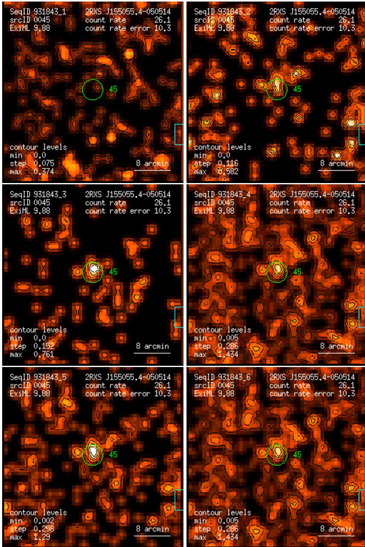
Figure 45: RASS 931843: detection 0045: band rate images, Gaussian filter: (1) PSPC channels 11 – 41, (2) 52 – 90, (3) 91 – 201, (4) 11 – 235, (5) 52 – 201, (6) 11 – 201. Broad band rates in counts/ks. Band rate contour levels in counts/ks/arcmin 2 .
