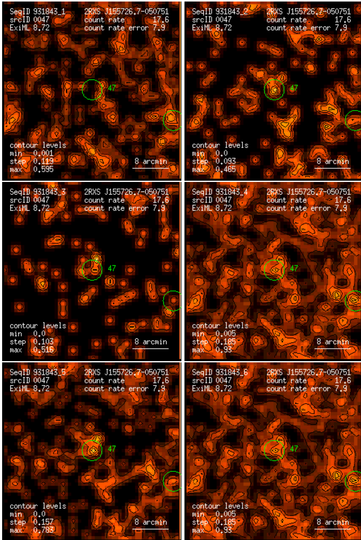
Figure 47: RASS 931843: detection 0047: band rate images, Gaussian filter: (1) PSPC channels 11 – 41, (2) 52 – 90, (3) 91 – 201, (4) 11 – 235, (5) 52 – 201, (6) 11 – 201. Broad band rates in counts/ks. Band rate contour levels in counts/ks/arcmin 2 .
