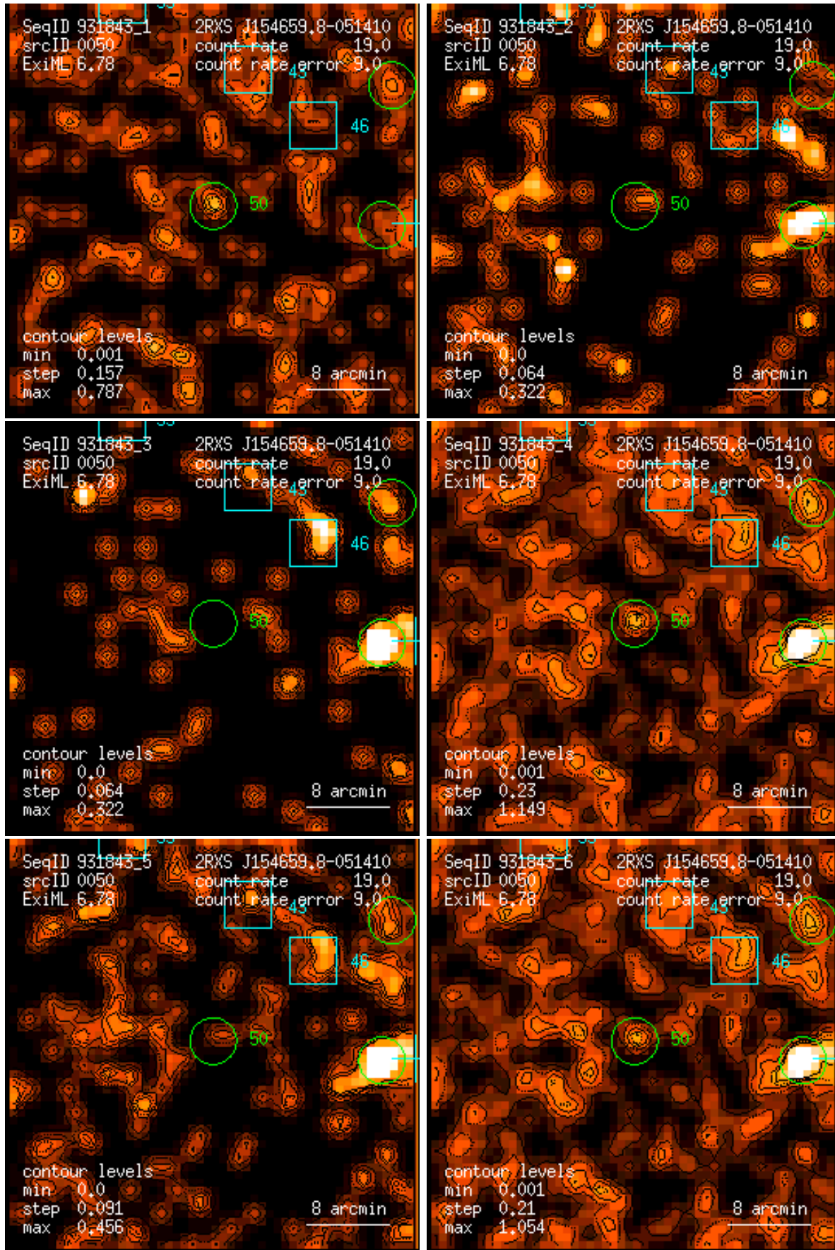
Figure 50: RASS 931843: detection 0050: band rate images, Gaussian filter: (1) PSPC channels 11 – 41, (2) 52 – 90, (3) 91 – 201, (4) 11 – 235, (5) 52 – 201, (6) 11 – 201. Broad band rates in counts/ks. Band rate contour levels in counts/ks/arcmin 2 .
