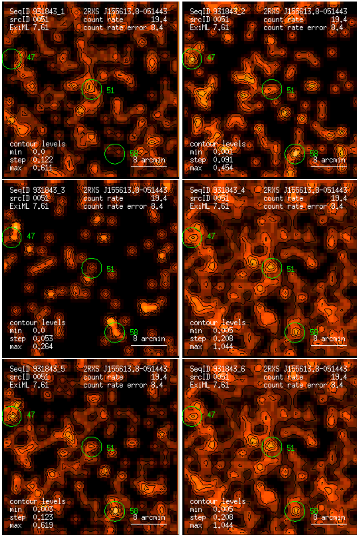
Figure 51: RASS 931843: detection 0051: band rate images, Gaussian filter: (1) PSPC channels 11 – 41, (2) 52 – 90, (3) 91 – 201, (4) 11 – 235, (5) 52 – 201, (6) 11 – 201. Broad band rates in counts/ks. Band rate contour levels in counts/ks/arcmin 2 .
