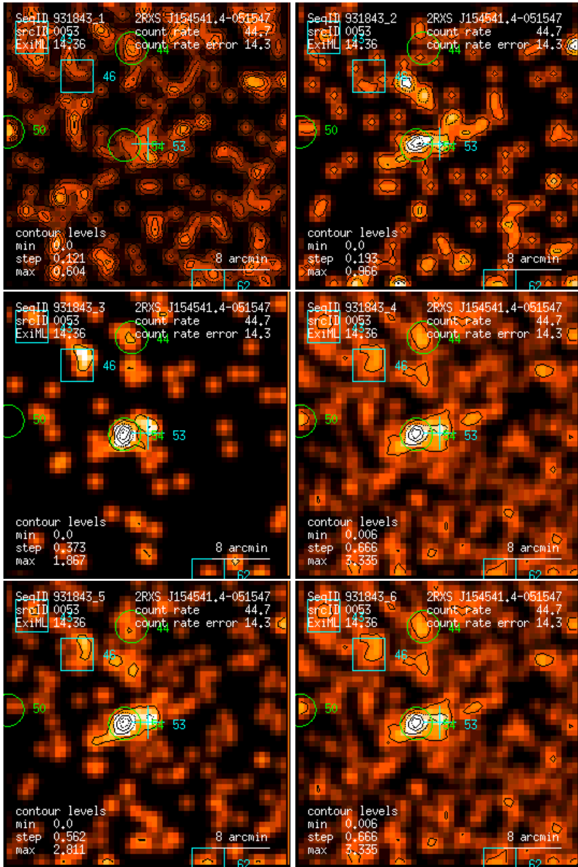
Figure 53: RASS 931843: detection 0053: band rate images, Gaussian filter: (1) PSPC channels 11 – 41, (2) 52 – 90, (3) 91 – 201, (4) 11 – 235, (5) 52 – 201, (6) 11 – 201. Broad band rates in counts/ks. Band rate contour levels in counts/ks/arcmin 2 .
