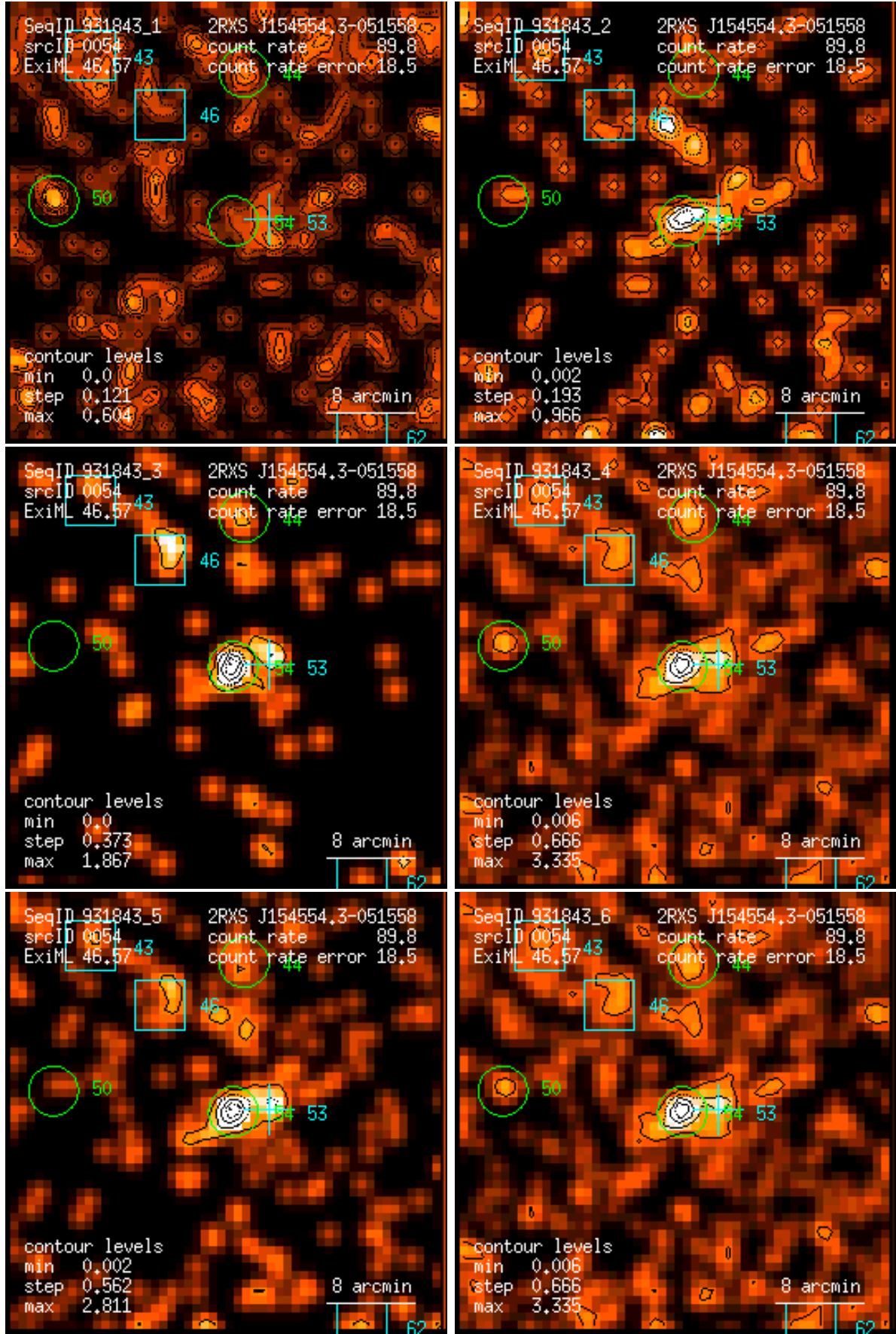
Figure 54: RASS 931843: detection 0054: band rate images, Gaussian filter: (1) PSPC channels 11 – 41, (2) 52 – 90, (3) 91 – 201, (4) 11 – 235, (5) 52 – 201, (6) 11 – 201. Broad band rates in counts/ks. Band rate contour levels in counts/ks/arcmin 2 .
