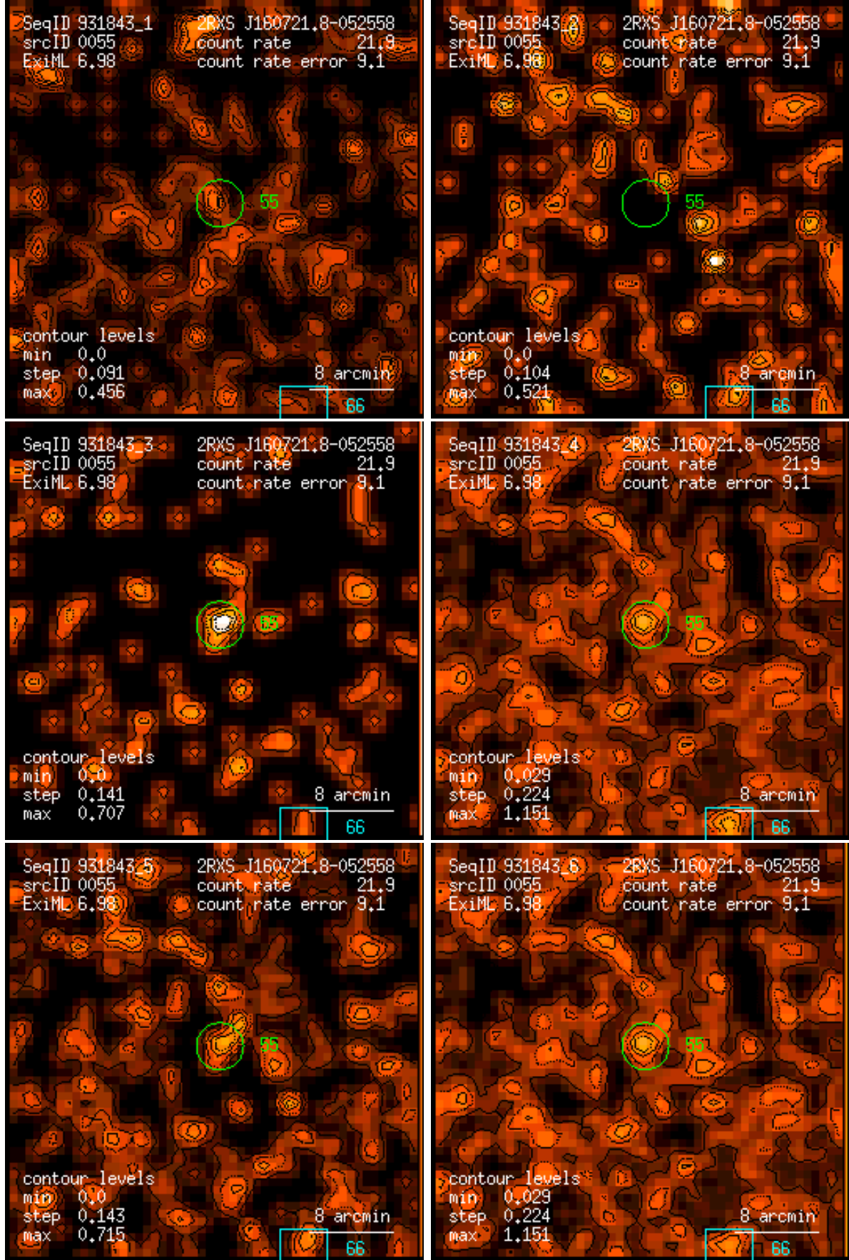
Figure 55: RASS 931843: detection 0055: band rate images, Gaussian filter: (1) PSPC channels 11 – 41, (2) 52 – 90, (3) 91 – 201, (4) 11 – 235, (5) 52 – 201, (6) 11 – 201. Broad band rates in counts/ks. Band rate contour levels in counts/ks/arcmin 2 .
