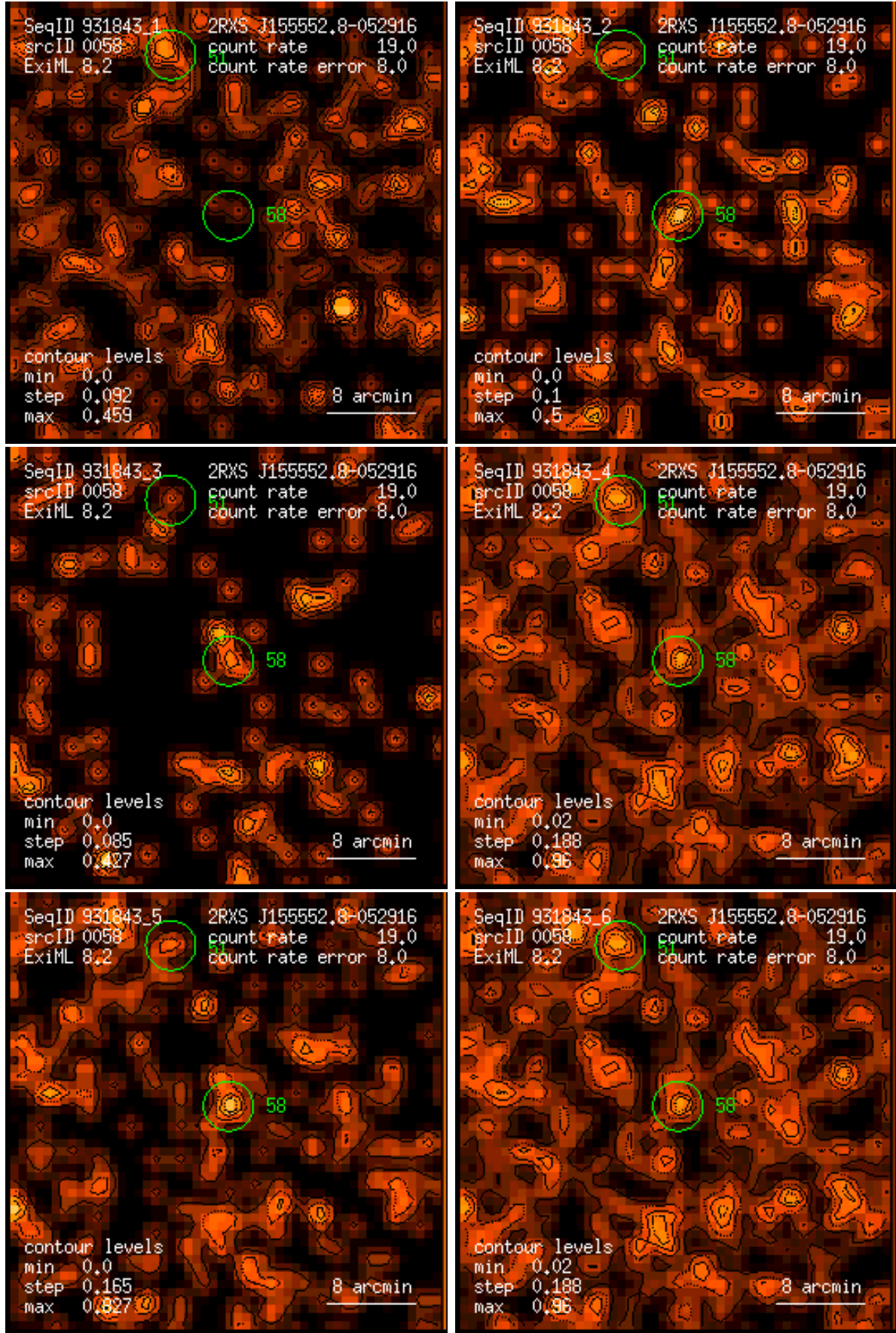
Figure 58: RASS 931843: detection 0058: band rate images, Gaussian filter: (1) PSPC channels 11 – 41, (2) 52 – 90, (3) 91 – 201, (4) 11 – 235, (5) 52 – 201, (6) 11 – 201. Broad band rates in counts/ks. Band rate contour levels in counts/ks/arcmin 2 .
