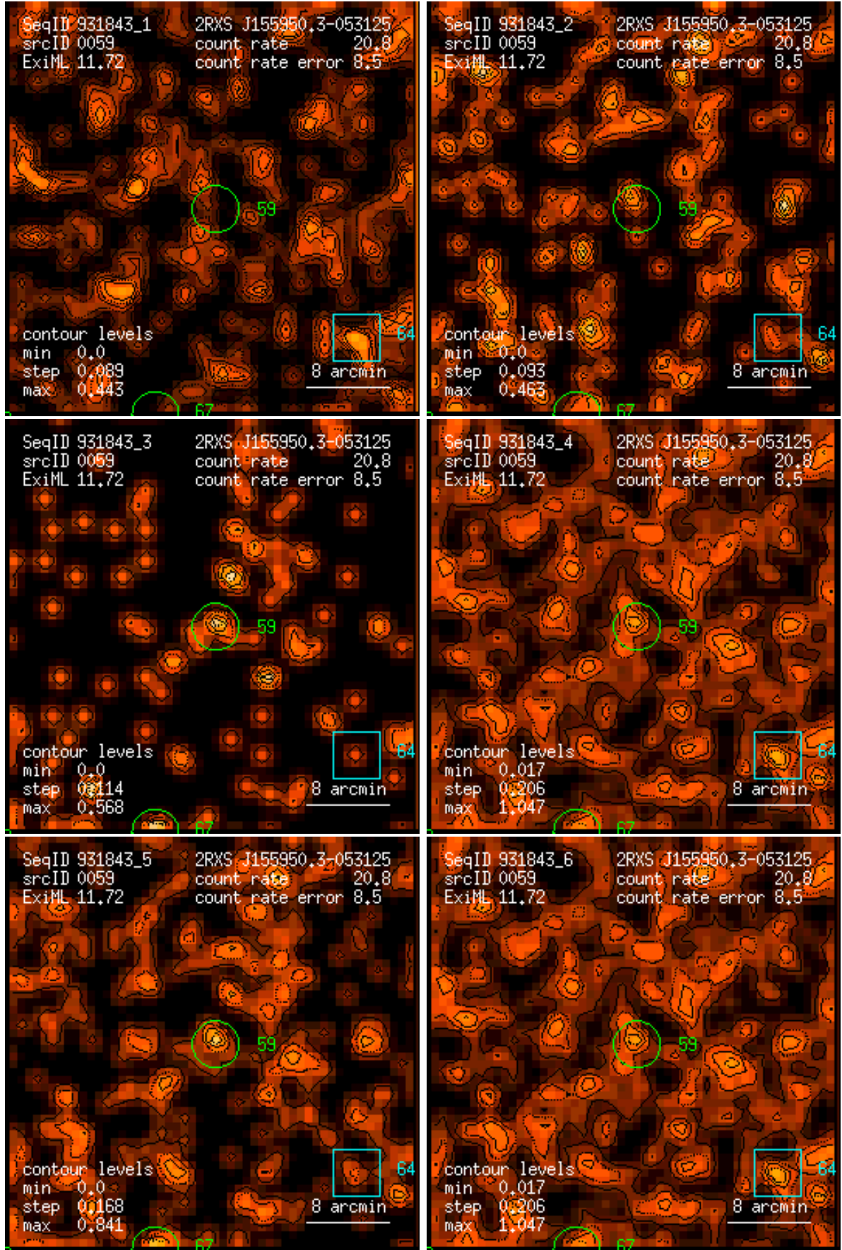
Figure 59: RASS 931843: detection 0059: band rate images, Gaussian filter: (1) PSPC channels 11 – 41, (2) 52 – 90, (3) 91 – 201, (4) 11 – 235, (5) 52 – 201, (6) 11 – 201. Broad band rates in counts/ks. Band rate contour levels in counts/ks/arcmin 2 .
