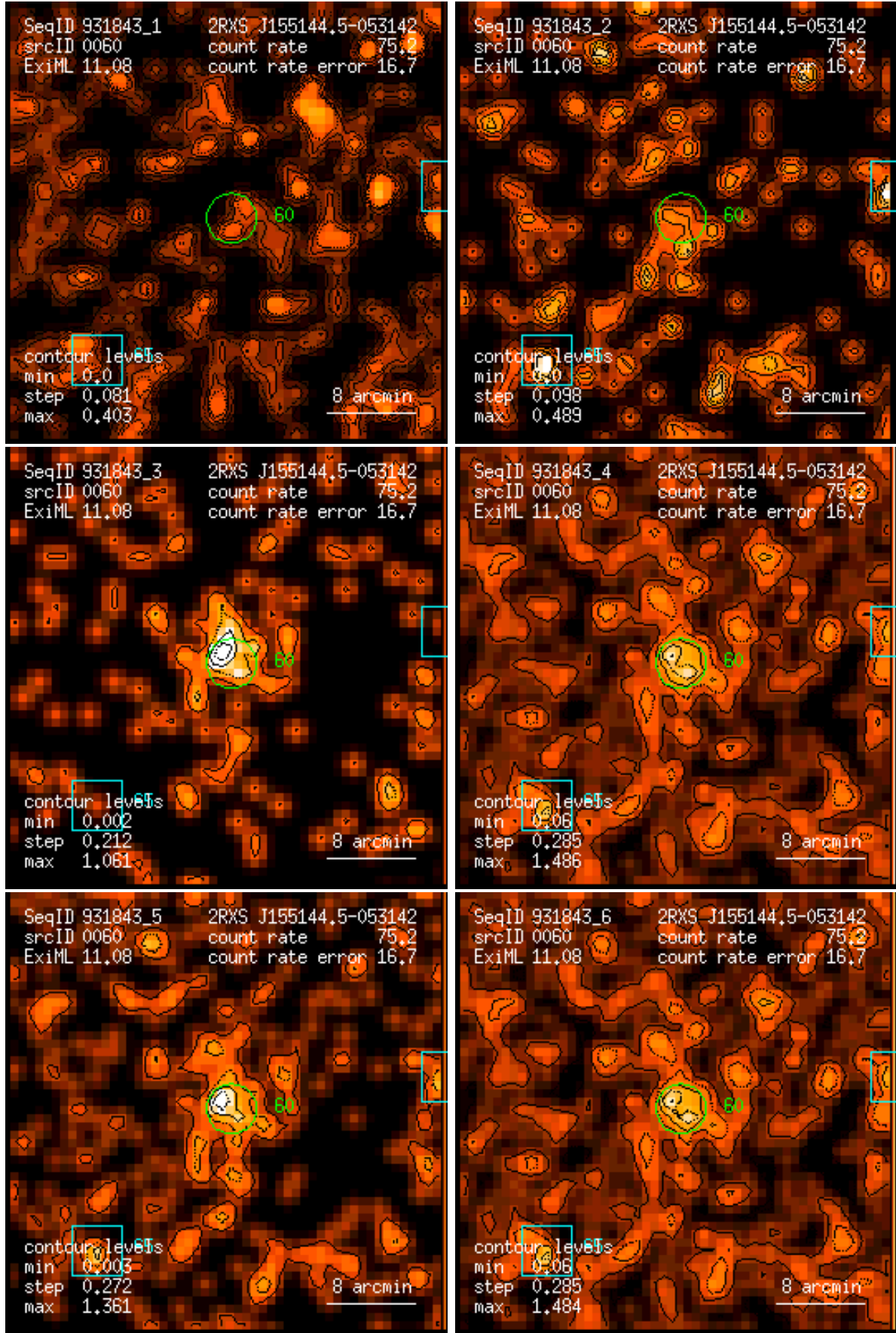
Figure 60: RASS 931843: detection 0060: band rate images, Gaussian filter: (1) PSPC channels 11 – 41, (2) 52 – 90, (3) 91 – 201, (4) 11 – 235, (5) 52 – 201, (6) 11 – 201. Broad band rates in counts/ks. Band rate contour levels in counts/ks/arcmin 2 .
