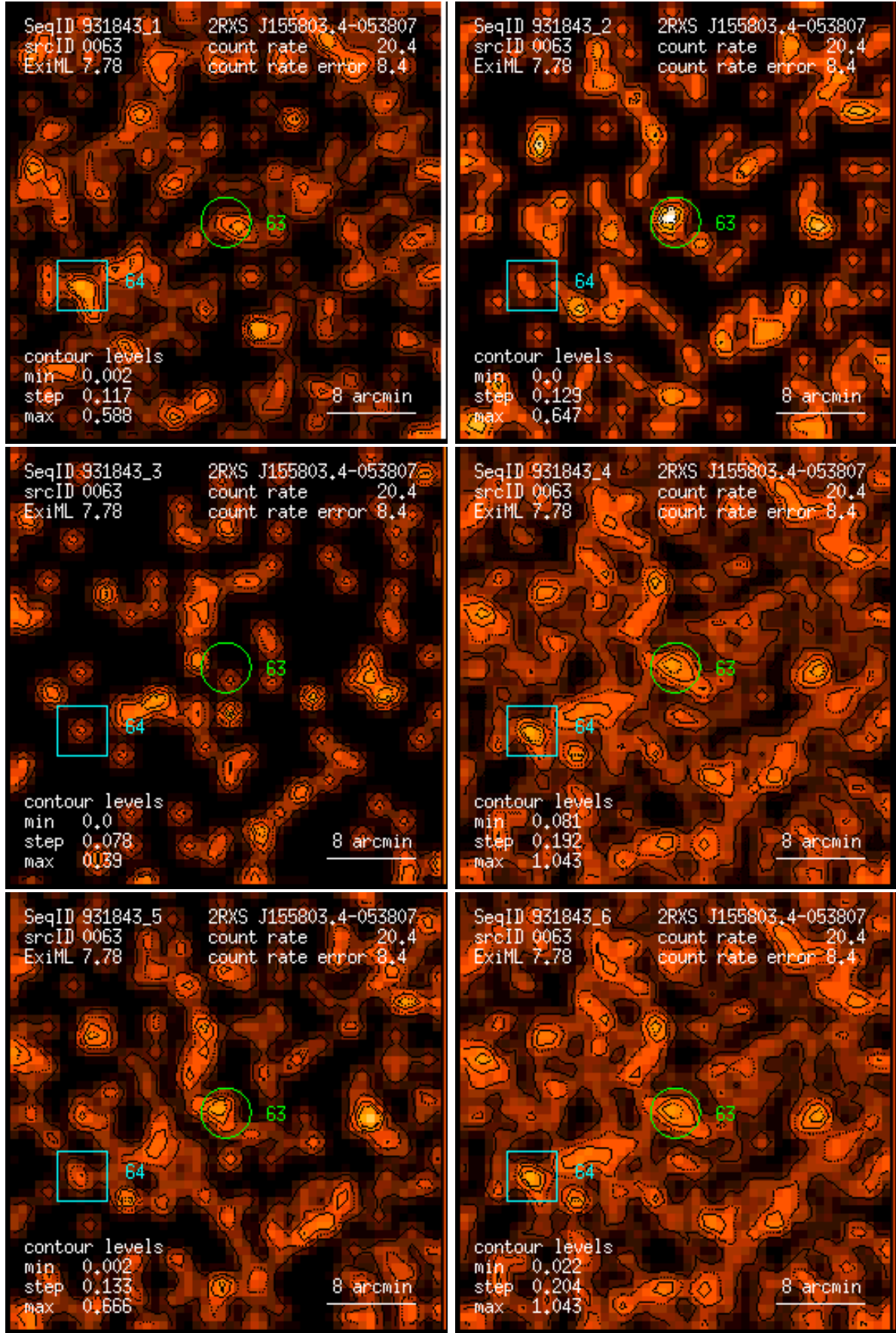
Figure 63: RASS 931843: detection 0063: band rate images, Gaussian filter: (1) PSPC channels 11 – 41, (2) 52 – 90, (3) 91 – 201, (4) 11 – 235, (5) 52 – 201, (6) 11 – 201. Broad band rates in counts/ks. Band rate contour levels in counts/ks/arcmin 2 .
