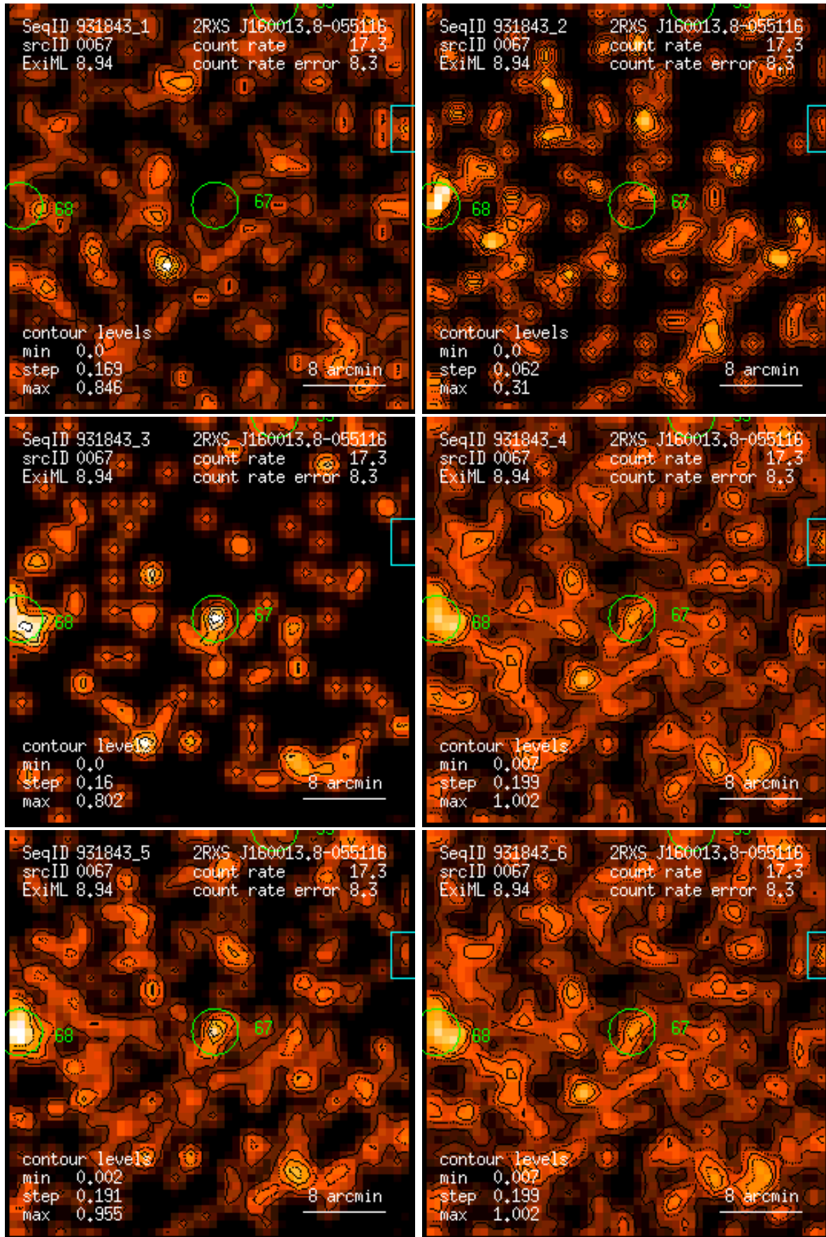
Figure 67: RASS 931843: detection 0067: band rate images, Gaussian filter: (1) PSPC channels 11 – 41, (2) 52 – 90, (3) 91 – 201, (4) 11 – 235, (5) 52 – 201, (6) 11 – 201. Broad band rates in counts/ks. Band rate contour levels in counts/ks/arcmin 2 .
