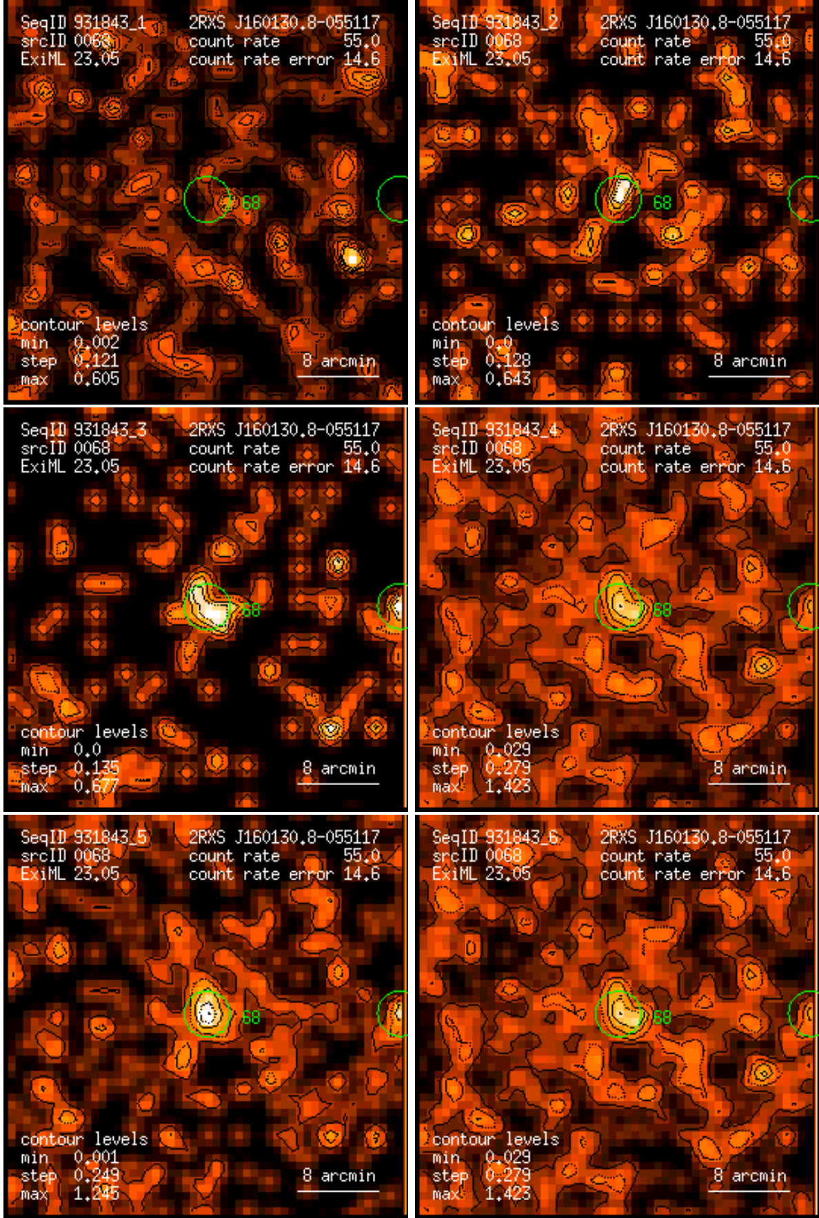
Figure 68: RASS 931843: detection 0068: band rate images, Gaussian filter: (1) PSPC channels 11 – 41, (2) 52 – 90, (3) 91 – 201, (4) 11 – 235, (5) 52 – 201, (6) 11 – 201. Broad band rates in counts/ks. Band rate contour levels in counts/ks/arcmin 2 .
