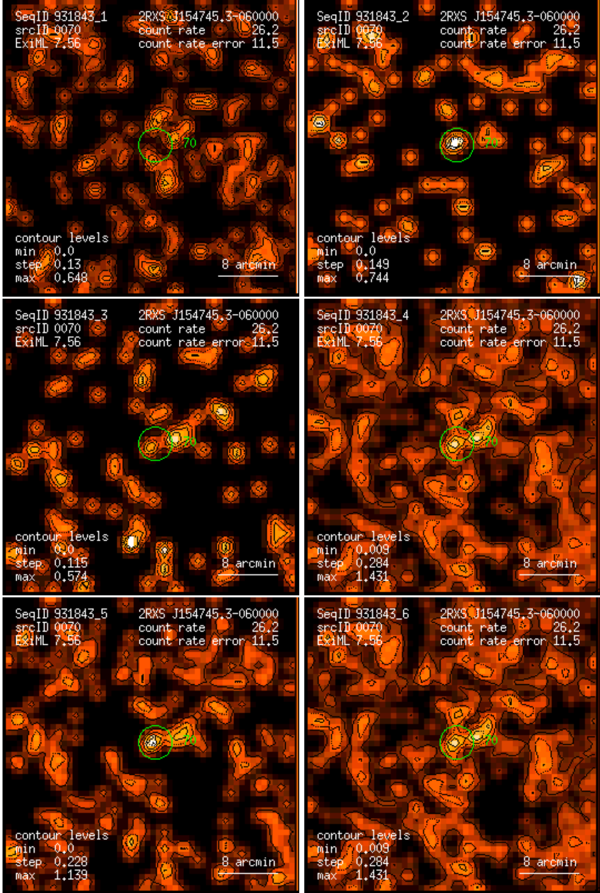
Figure 70: RASS 931843: detection 0070: band rate images, Gaussian filter: (1) PSPC channels 11 – 41, (2) 52 – 90, (3) 91 – 201, (4) 11 – 235, (5) 52 – 201, (6) 11 – 201. Broad band rates in counts/ks. Band rate contour levels in counts/ks/arcmin 2 .
