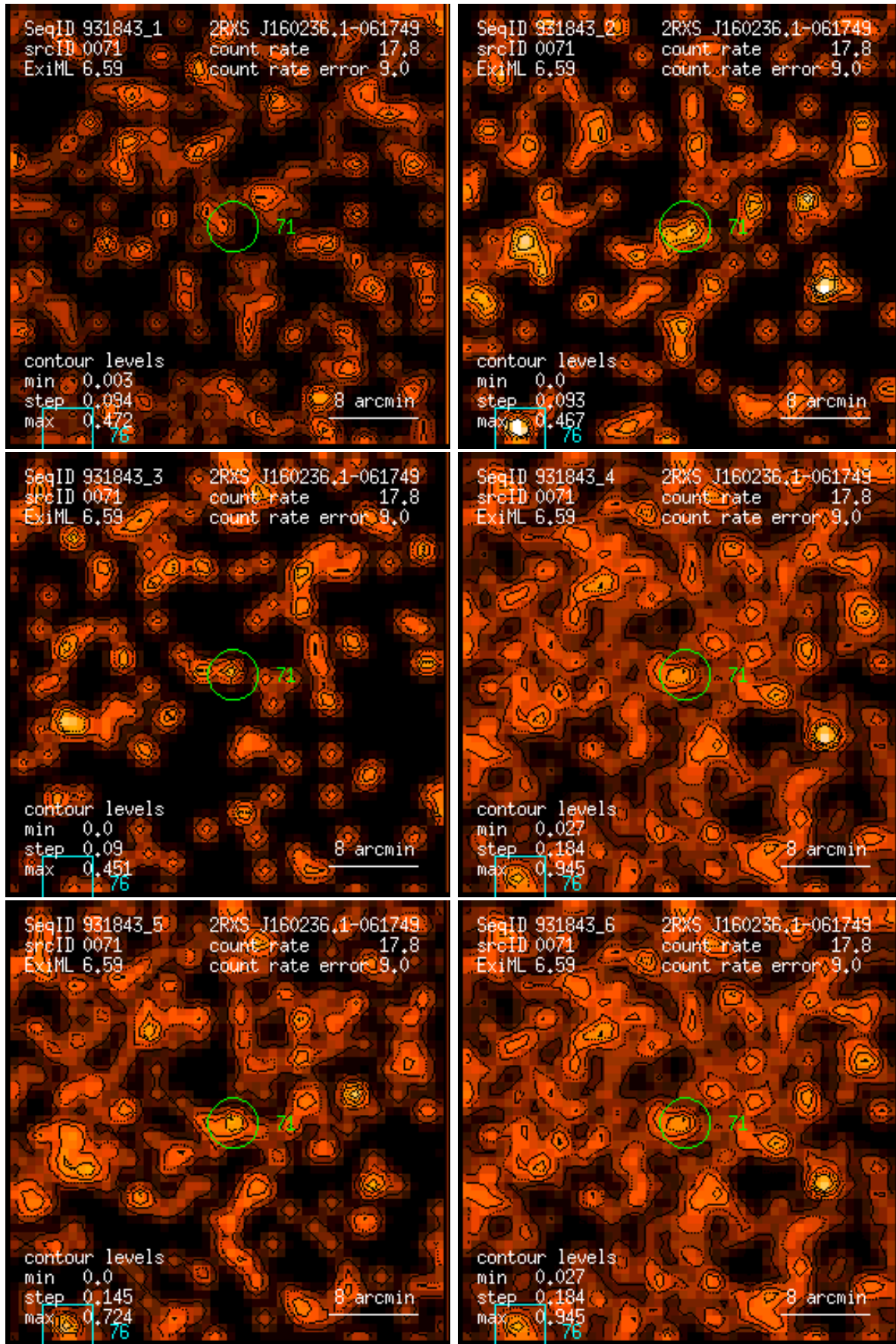
Figure 71: RASS 931843: detection 0071: band rate images, Gaussian filter: (1) PSPC channels 11 – 41, (2) 52 – 90, (3) 91 – 201, (4) 11 – 235, (5) 52 – 201, (6) 11 – 201. Broad band rates in counts/ks. Band rate contour levels in counts/ks/arcmin 2 .
