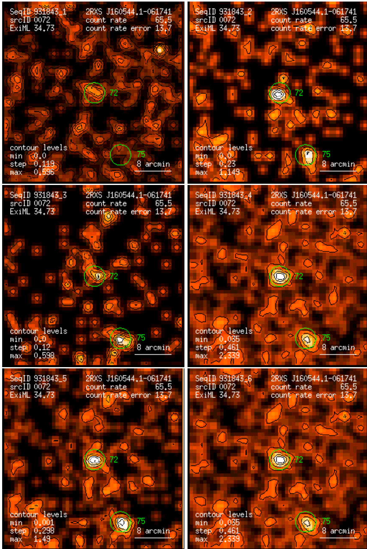
Figure 72: RASS 931843: detection 0072: band rate images, Gaussian filter: (1) PSPC channels 11 – 41, (2) 52 – 90, (3) 91 – 201, (4) 11 – 235, (5) 52 – 201, (6) 11 – 201. Broad band rates in counts/ks. Band rate contour levels in counts/ks/arcmin 2 .
