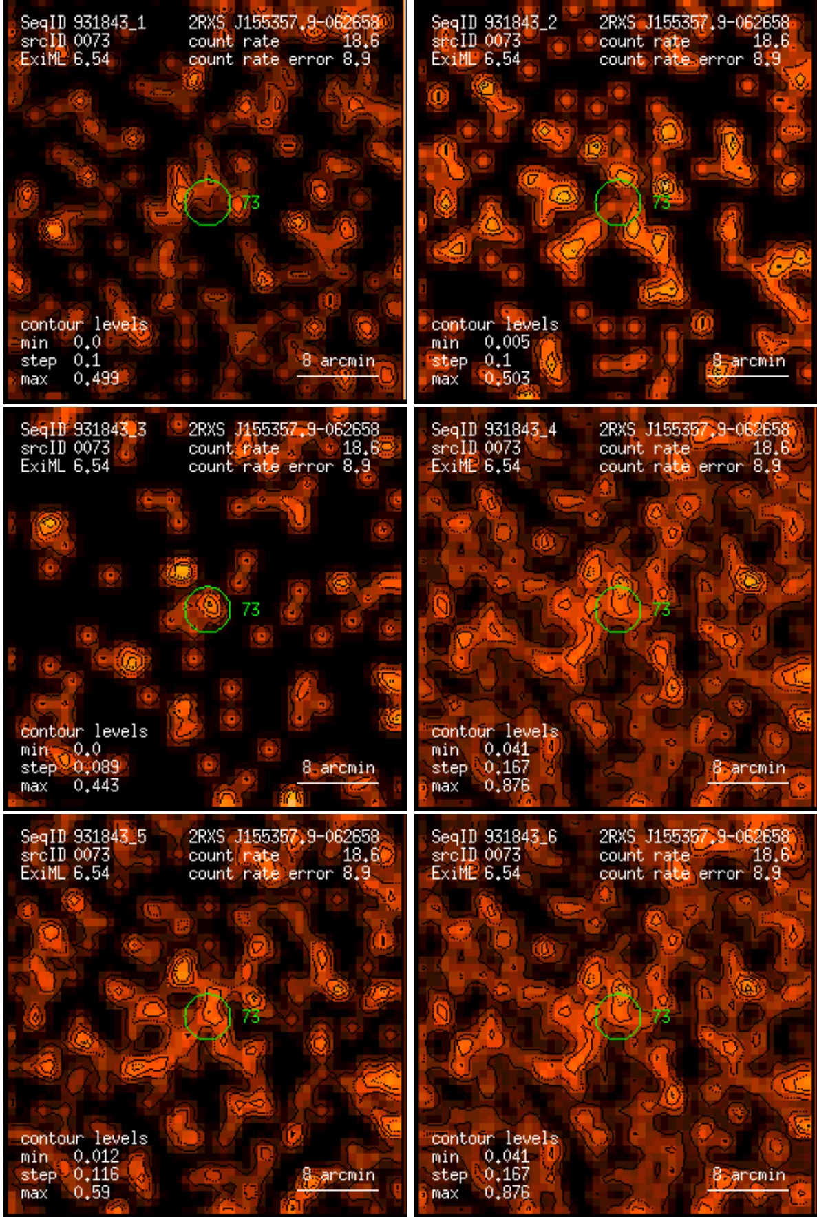
Figure 73: RASS 931843: detection 0073: band rate images, Gaussian filter: (1) PSPC channels 11 – 41, (2) 52 – 90, (3) 91 – 201, (4) 11 – 235, (5) 52 – 201, (6) 11 – 201. Broad band rates in counts/ks. Band rate contour levels in counts/ks/arcmin 2 .
