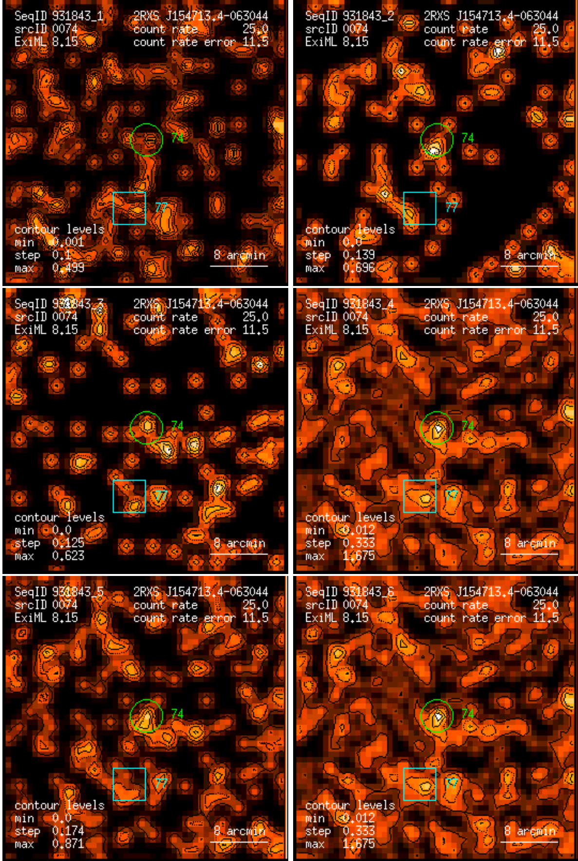
Figure 74: RASS 931843: detection 0074: band rate images, Gaussian filter: (1) PSPC channels 11 – 41, (2) 52 – 90, (3) 91 – 201, (4) 11 – 235, (5) 52 – 201, (6) 11 – 201. Broad band rates in counts/ks. Band rate contour levels in counts/ks/arcmin 2 .
