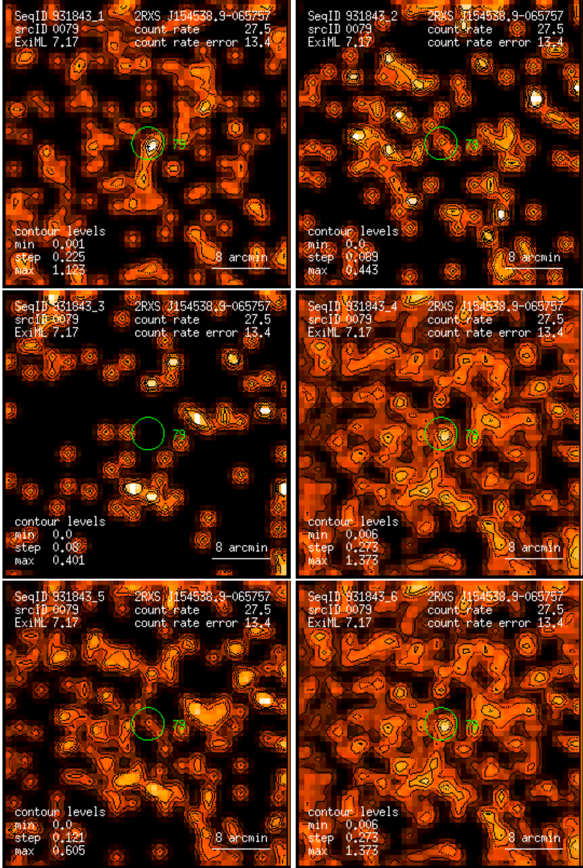
Figure 79: RASS 931843: detection 0079: band rate images, Gaussian filter: (1) PSPC channels 11 – 41, (2) 52 – 90, (3) 91 – 201, (4) 11 – 235, (5) 52 – 201, (6) 11 – 201. Broad band rates in counts/ks. Band rate contour levels in counts/ks/arcmin 2 .
