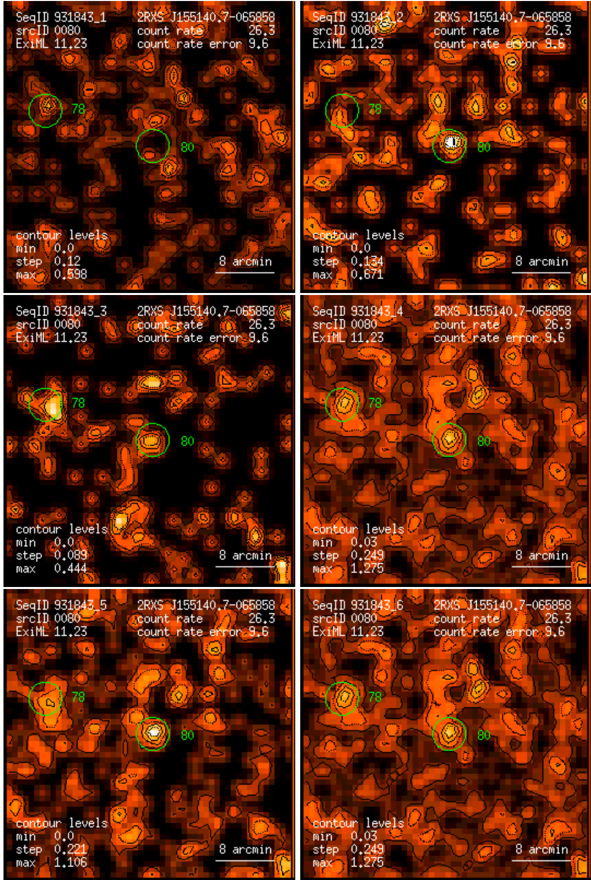
Figure 80: RASS 931843: detection 0080: band rate images, Gaussian filter: (1) PSPC channels 11 – 41, (2) 52 – 90, (3) 91 – 201, (4) 11 – 235, (5) 52 – 201, (6) 11 – 201. Broad band rates in counts/ks. Band rate contour levels in counts/ks/arcmin 2 .
