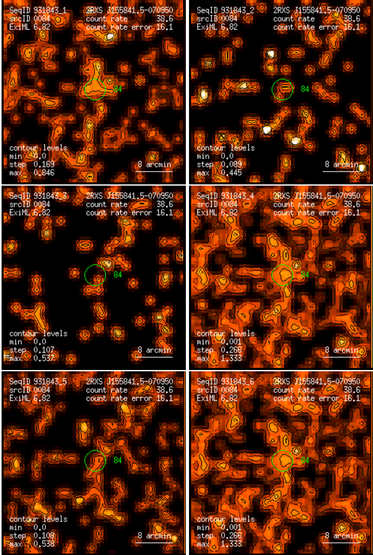
Figure 84: RASS 931843: detection 0084: band rate images, Gaussian filter: (1) PSPC channels 11 – 41, (2) 52 – 90, (3) 91 – 201, (4) 11 – 235, (5) 52 – 201, (6) 11 – 201. Broad band rates in counts/ks. Band rate contour levels in counts/ks/arcmin 2 .
