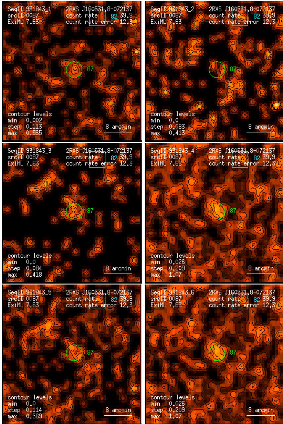
Figure 87: RASS 931843: detection 0087: band rate images, Gaussian filter: (1) PSPC channels 11 – 41, (2) 52 – 90, (3) 91 – 201, (4) 11 – 235, (5) 52 – 201, (6) 11 – 201. Broad band rates in counts/ks. Band rate contour levels in counts/ks/arcmin 2 .
