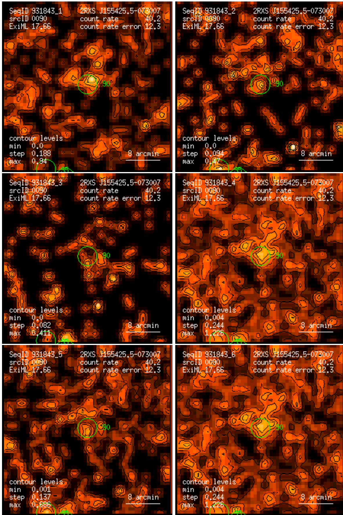
Figure 90: RASS 931843: detection 0090: band rate images, Gaussian filter: (1) PSPC channels 11 – 41, (2) 52 – 90, (3) 91 – 201, (4) 11 – 235, (5) 52 – 201, (6) 11 – 201. Broad band rates in counts/ks. Band rate contour levels in counts/ks/arcmin 2 .
