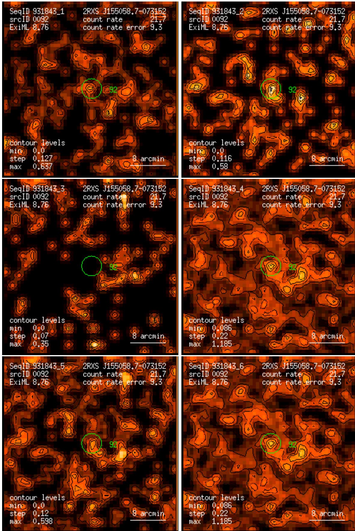
Figure 92: RASS 931843: detection 0092: band rate images, Gaussian filter: (1) PSPC channels 11 – 41, (2) 52 – 90, (3) 91 – 201, (4) 11 – 235, (5) 52 – 201, (6) 11 – 201. Broad band rates in counts/ks. Band rate contour levels in counts/ks/arcmin 2 .
