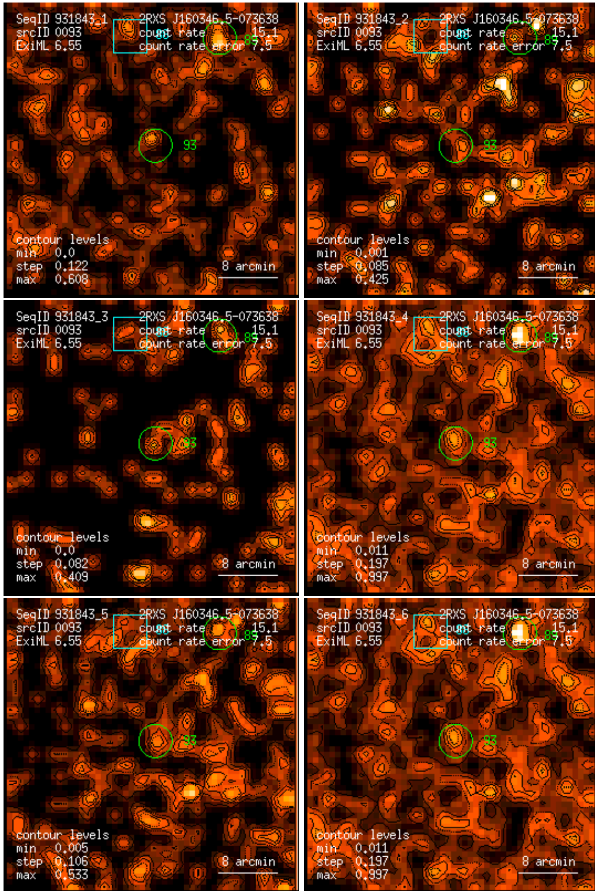
Figure 93: RASS 931843: detection 0093: band rate images, Gaussian filter: (1) PSPC channels 11 – 41, (2) 52 – 90, (3) 91 – 201, (4) 11 – 235, (5) 52 – 201, (6) 11 – 201. Broad band rates in counts/ks. Band rate contour levels in counts/ks/arcmin 2 .
