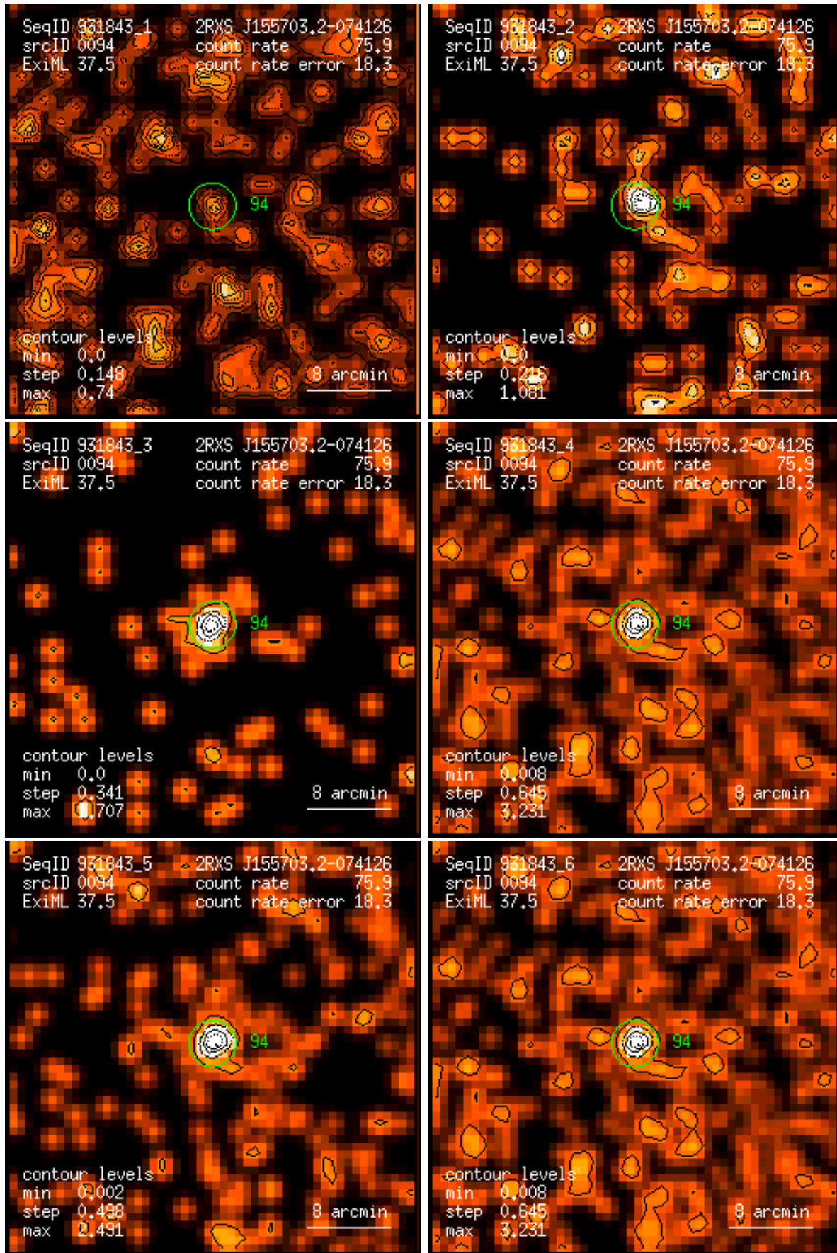
Figure 94: RASS 931843: detection 0094: band rate images, Gaussian filter: (1) PSPC channels 11 – 41, (2) 52 – 90, (3) 91 – 201, (4) 11 – 235, (5) 52 – 201, (6) 11 – 201. Broad band rates in counts/ks. Band rate contour levels in counts/ks/arcmin 2 .
