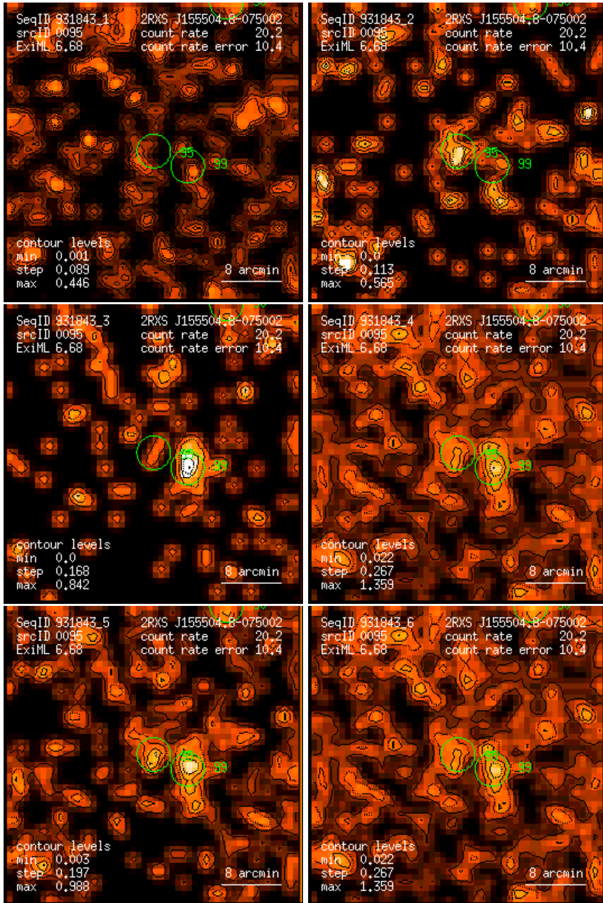
Figure 95: RASS 931843: detection 0095: band rate images, Gaussian filter: (1) PSPC channels 11 – 41, (2) 52 – 90, (3) 91 – 201, (4) 11 – 235, (5) 52 – 201, (6) 11 – 201. Broad band rates in counts/ks. Band rate contour levels in counts/ks/arcmin 2 .
