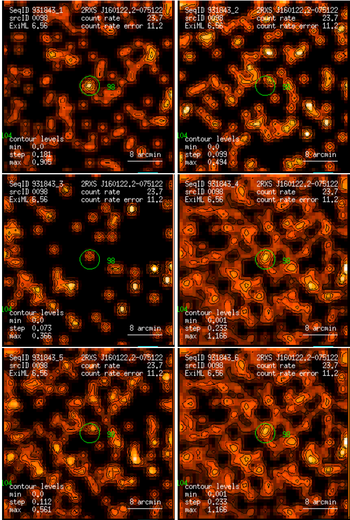
Figure 98: RASS 931843: detection 0098: band rate images, Gaussian filter: (1) PSPC channels 11 – 41, (2) 52 – 90, (3) 91 – 201, (4) 11 – 235, (5) 52 – 201, (6) 11 – 201. Broad band rates in counts/ks. Band rate contour levels in counts/ks/arcmin 2 .
