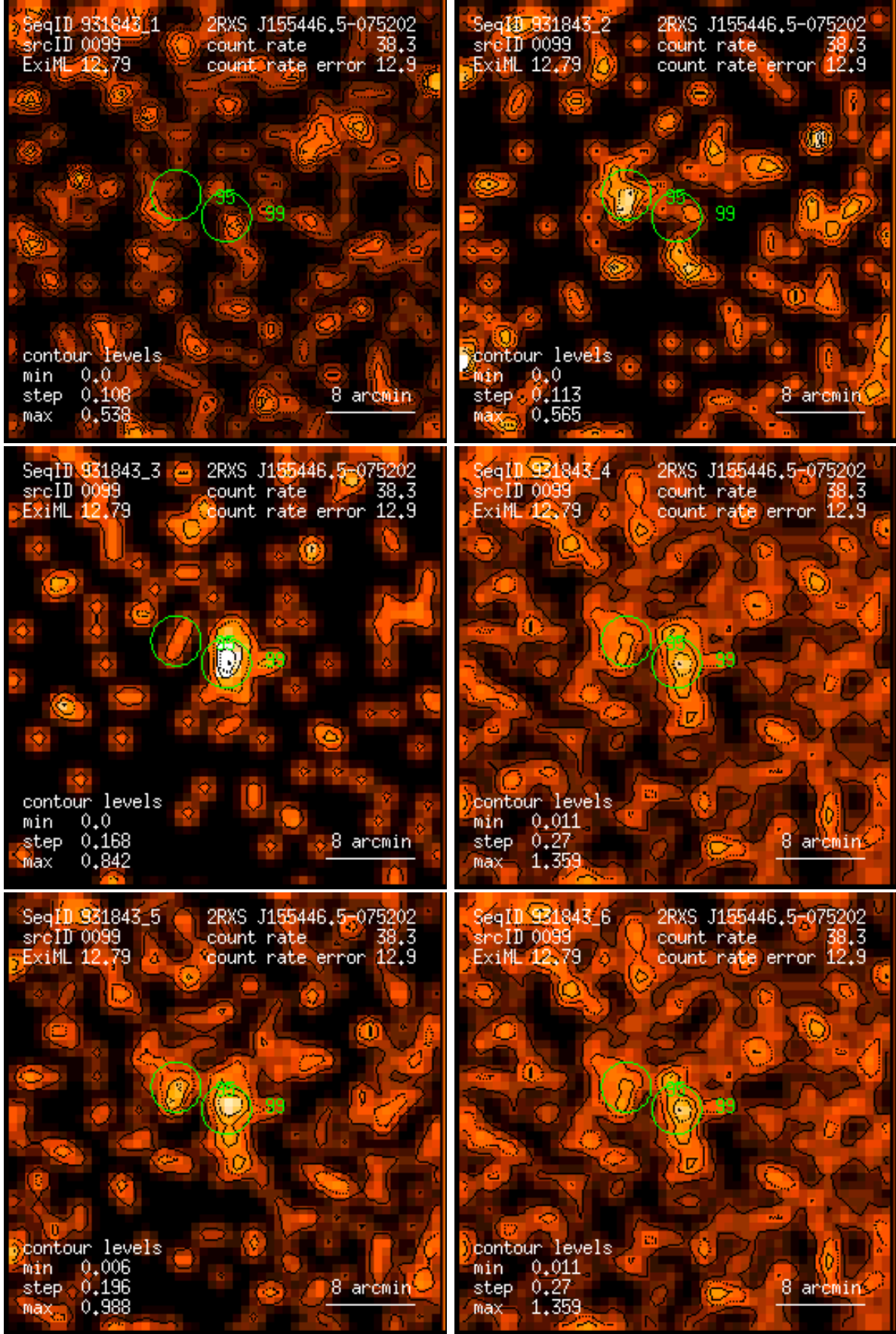
Figure 99: RASS 931843: detection 0099: band rate images, Gaussian filter: (1) PSPC channels 11 – 41, (2) 52 – 90, (3) 91 – 201, (4) 11 – 235, (5) 52 – 201, (6) 11 – 201. Broad band rates in counts/ks. Band rate contour levels in counts/ks/arcmin 2 .
