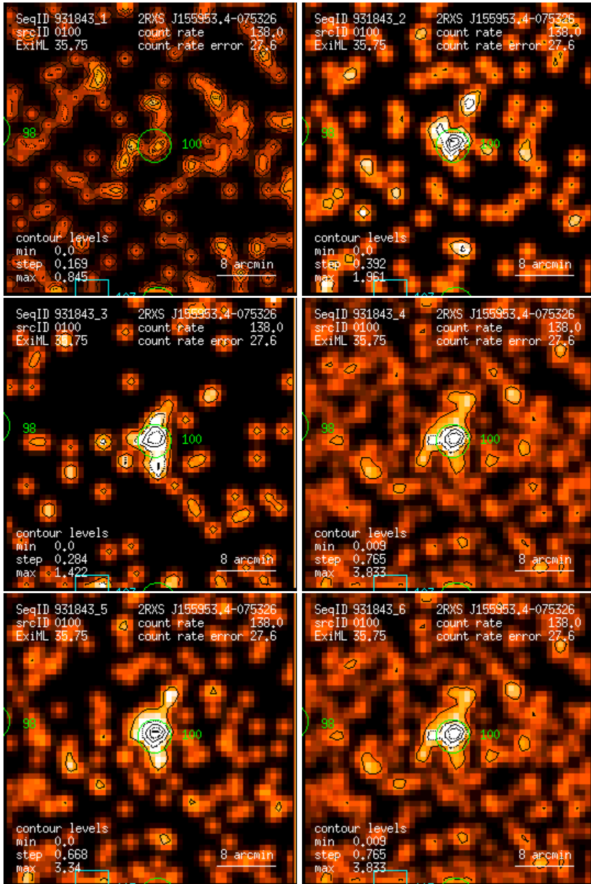
Figure 100: RASS 931843: detection 0100: band rate images, Gaussian filter: (1) PSPC channels 11 – 41, (2) 52 – 90, (3) 91 – 201, (4) 11 – 235, (5) 52 – 201, (6) 11 – 201. Broad band rates in counts/ks. Band rate contour levels in counts/ks/arcmin 2 .
