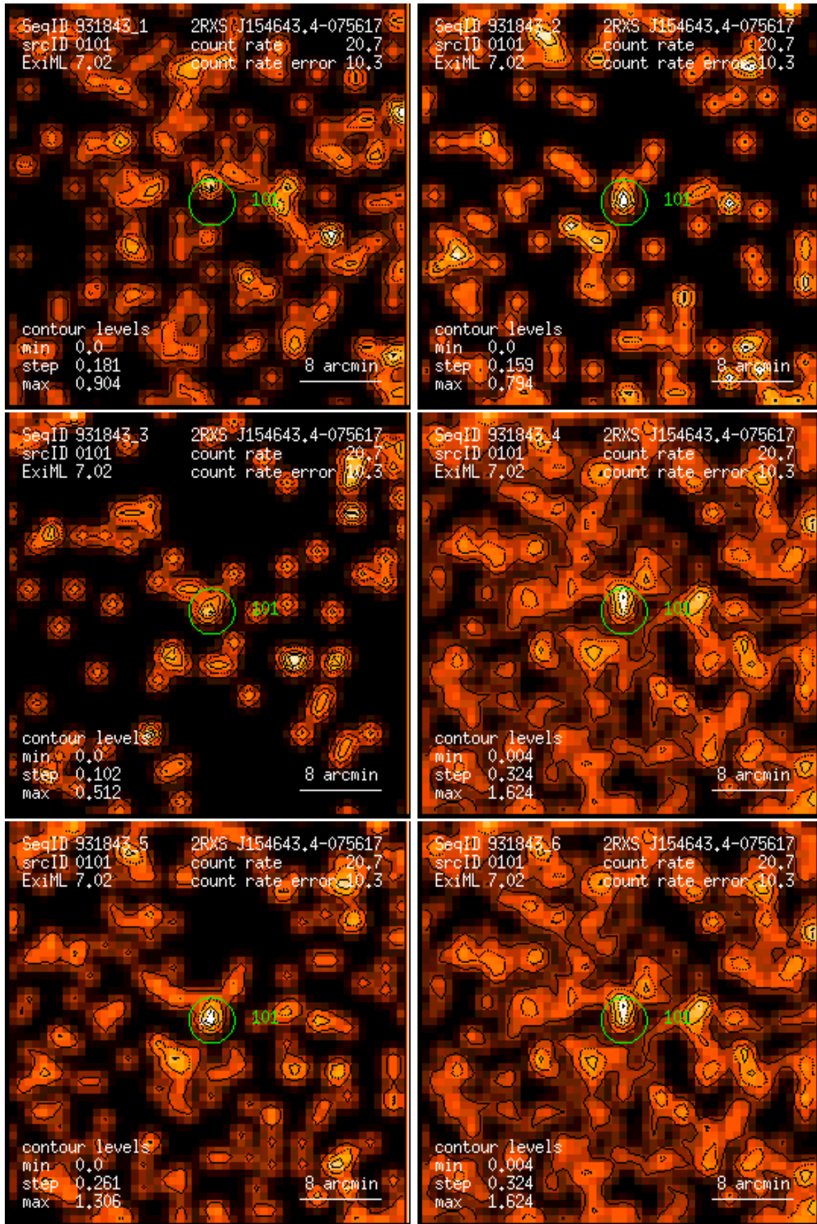
Figure 101: RASS 931843: detection 0101: band rate images, Gaussian filter: (1) PSPC channels 11 – 41, (2) 52 – 90, (3) 91 – 201, (4) 11 – 235, (5) 52 – 201, (6) 11 – 201. Broad band rates in counts/ks. Band rate contour levels in counts/ks/arcmin 2 .
